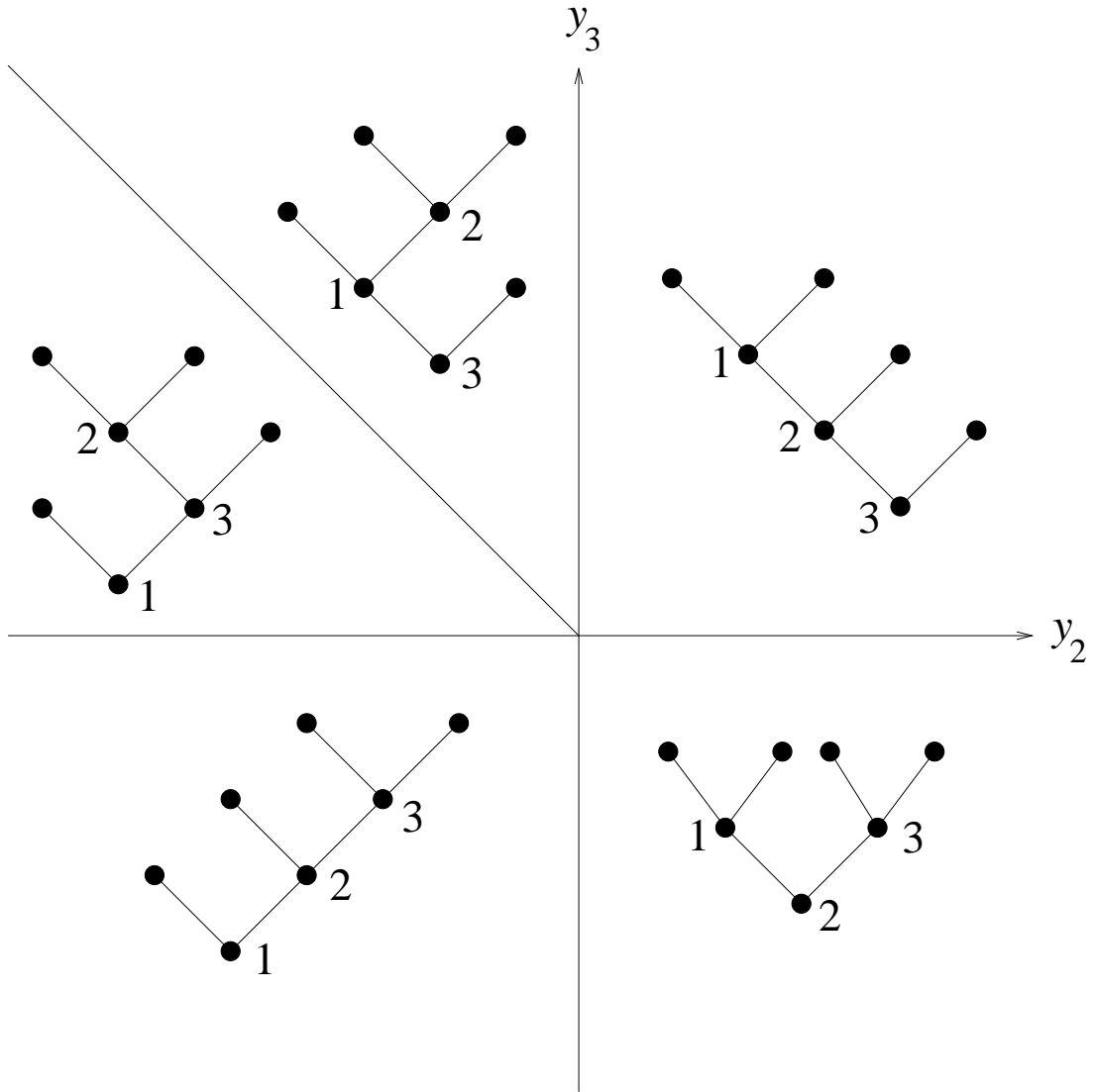
Figure 8: The fan \mathbf{F}_3
