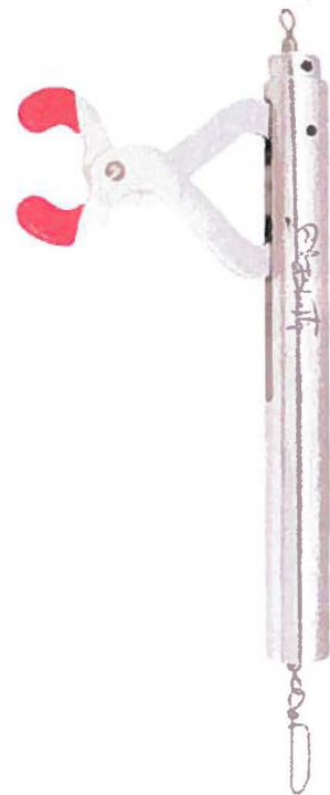
Blacktip Catch and Release Recompression Tool (the Git-R-Down) ( www.git-r-down.com )
