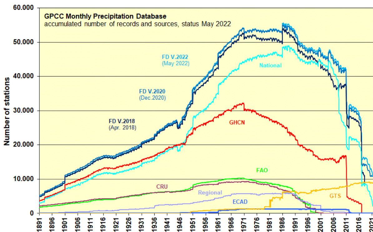
Figure 8: Total number of stations with monthly precipitation data in GPCC's full database according to the different data sources
