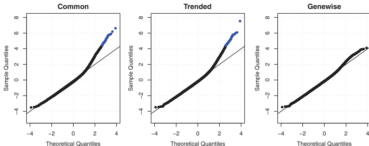
Figure 2. QQ-plots of goodness of fit statistics using common, trended or empirical Bayes genewise (tagwise) dispersions. Genewise deviance statistics were transformed to normality, and plotted against theoretical normal quantiles. Points in blue are those genes with a significantly poor fit (Holm-adjusted P -value < 0.05 ). When using genewise dispersions, no genes show a significantly poor fit.
