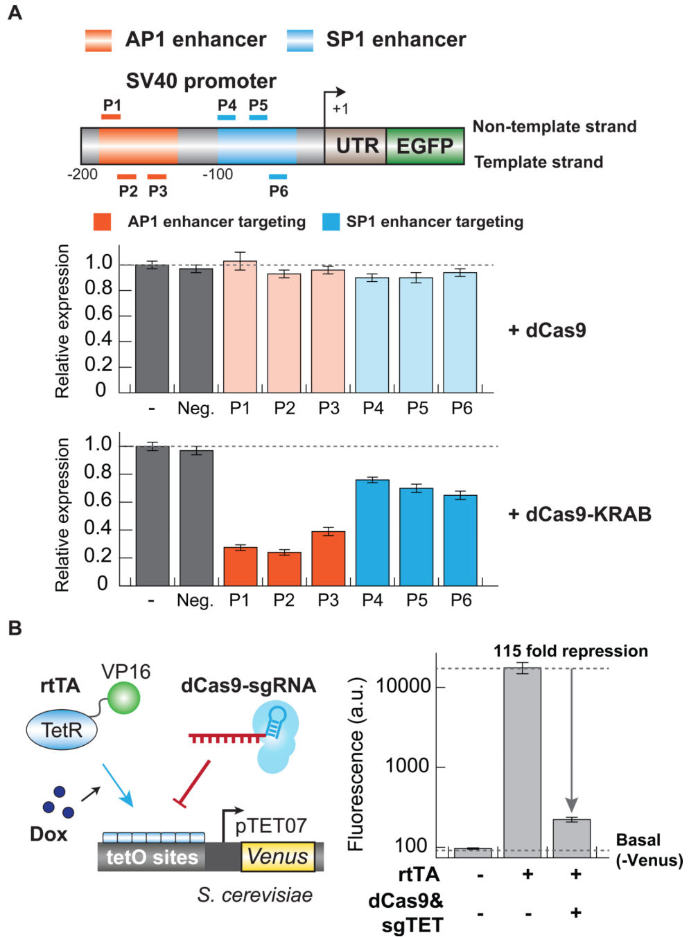
Figure 4. CRISPRi can suppress gene expression from the promoter of a gene (A) A dCas9-KRAB fusion protein efficiently silences GFP expression when targeted to the SV40 promoter of an SV40-GFP reporter. 6 sgRNAs targeting different regions of the SV40 promoter as indicated are transfected into GFP+HEK293 cells stably expressing either dCas9 (upper panel) or dCas9-KRAB (lower panel). GFP fluorescence is quantified by flow cytometry 6 days following transfection and displayed as signal normalized to a vector control. The data are displayed as mean \pm standard deviation for 3 independent experiments. (B) The dCas9 construct and an sgRNA (sgTET) construct were co-transformed into a yeast strain expressing a TetON-Venus reporter and the rtTA protein. Doxycycline was added to
