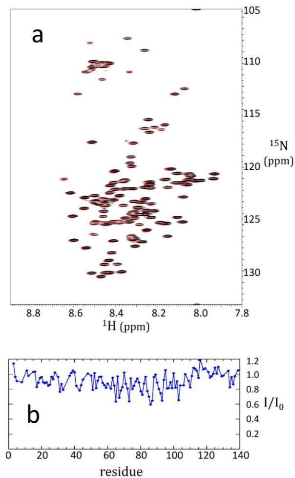
Figure S4. ^{15}\text{N} HSQC spectra of \alpha -syn at pH 7.4. (a) Overlaid NMR ^{15}\text{N} HSQC spectra of ^{13}\text{C}/^{15}\text{N} labeled \alpha -syn (40 \mu\text{M} , red) and in the presence of GCase (40 \mu\text{M} , black). (b) Plot of relative spectra intensity ratio of the \alpha -syn-GCase and \alpha -syn alone.
