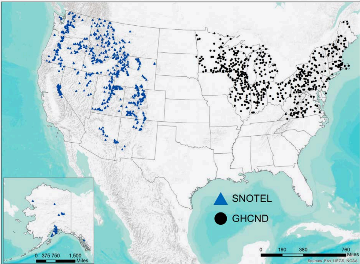
Figure A2. Global historical climatology network daily (GHCND) stations (black circles) and SNOW TElemetry (SNOTEL) network stations used in the high/low snow analysis.
