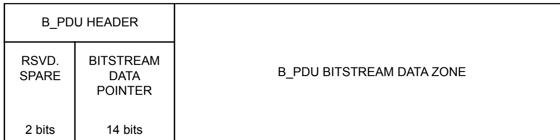
Figure 4-4: Bitstream Protocol Data Unit (B_PDU)
