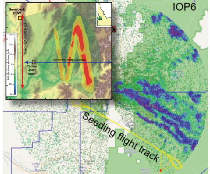
Hypothesized (left) and radar-observed effect of cloud seeding in SNOWIE
