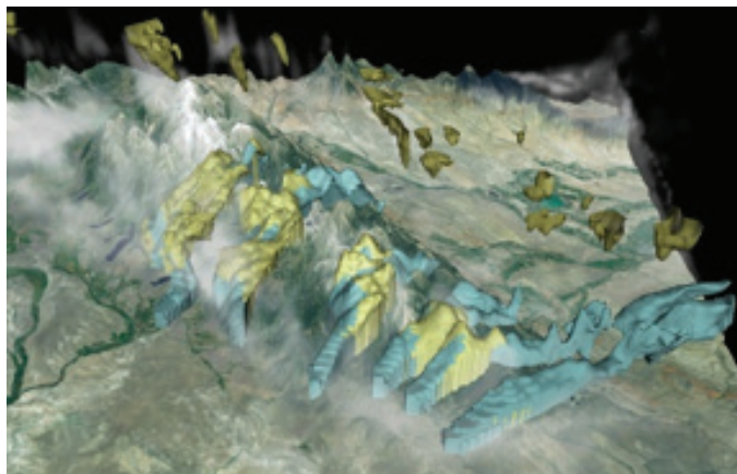
WRF-WxMod® simulation of clouds (white), ice (yellow) and AgI seeding plumes (blue).
