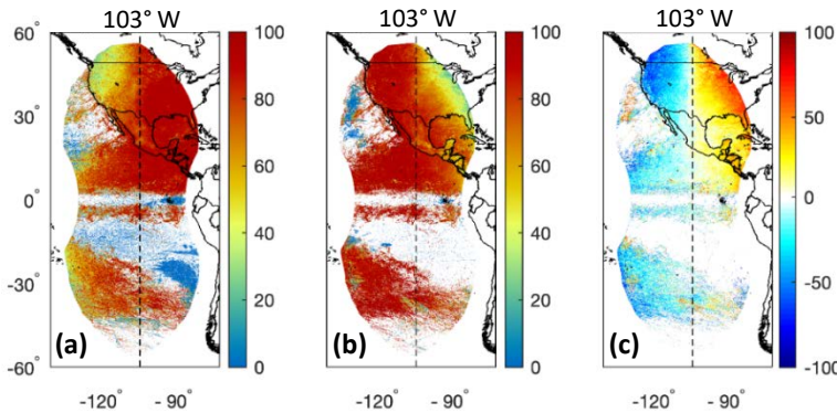
Panel a indicates the % of G17 flashes observed by G16 (and visa versa in panel b). Panel c illustrates the difference (i.e., panel a minus panel b) with warm (cool) colors in indicating G16 (G17) detects more flashes 1
