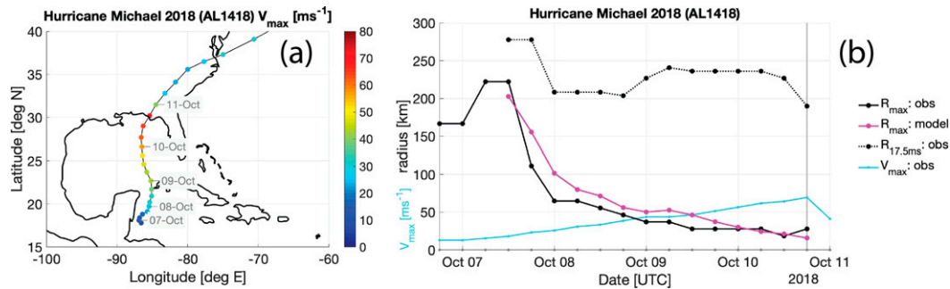
FIG. 7. Example application of our model to Hurricane Michael (2018). (a) Map of storm track with best track V_{max} (color dots); dates shown at 0000 UTC. (b) Predicted R_{max} (pink), EBT R_{max} (black solid), EBT R_{17.5ms} (black dashed), and V_{max} (light blue) prior to landfall (light gray line).
