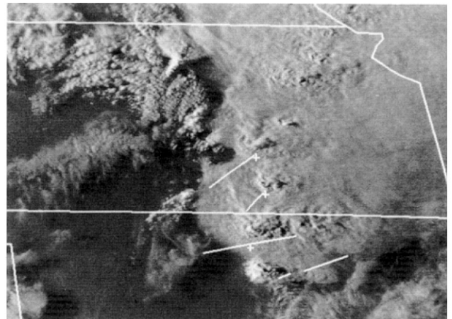
Figure 1. GOES-7 1 km resolution visible image taken at 6:05 PM, CST, on April 26, 1991. Ground tracks of major tornadoes have been added, with a + mark showing the approximate ground location of the tornado at the time of the image. Note that tornado activity has not yet begun with the southern most track.
