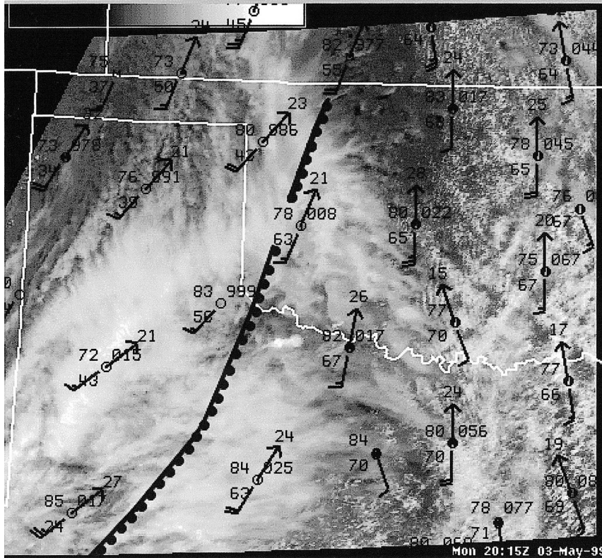
FIG. 13. GOES-8 visible satellite image at 2015 UTC 3 May 1999. Dryline position as shown by scalloped line. Station plots are U.S. convention except that wind gusts (kt) are indicated by arrows.
