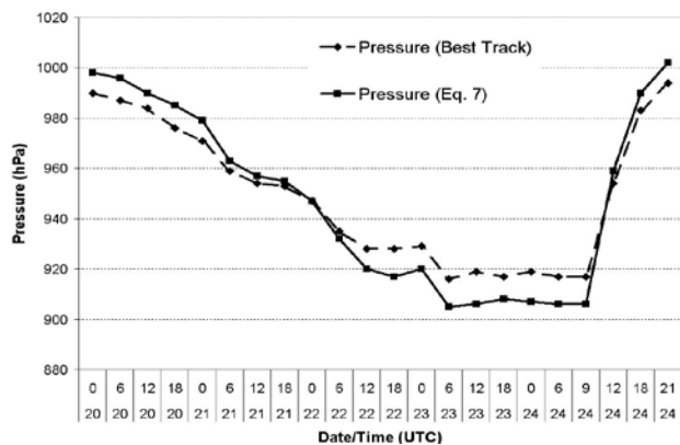
Fig. 6(b) Comparison of central pressure for TC Monica (April 2006) between the Australian best track and Eqn 7 in the central region (Darwin TCWC) where Love and Murphy (1985) WPR is used.
