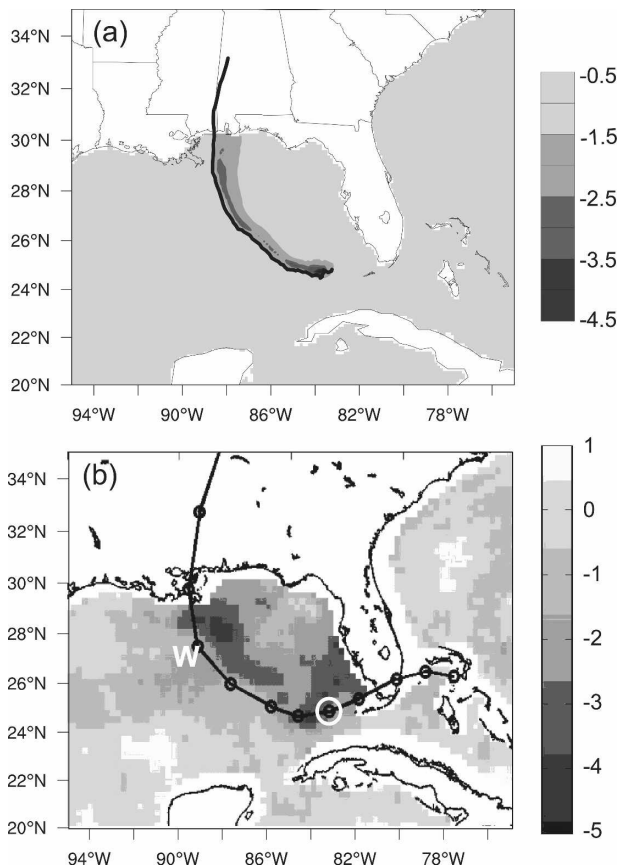
FIG. 8. (a) Change in SST ( ^\circ\text{C} ) produced during a 72-h three-domain simulation using AHW (same configuration as for 1.33-km nest in Fig. 5) coupled to the mixed layer ocean model with h_0 = 30 \text{ m} and \Gamma = 0.14 \text{ K m}^{-1} . Storm track is also indicated; (b) SST ( ^\circ\text{C} ) difference (31 Aug minus 25 Aug) derived from daily composite Tropical Rainfall Measuring Mission–Advanced Microwave Scanning Radiometer (TRMM–AMS) data and observed storm track (black line) with 12-hourly positions indicated with circles. “W” in (b) indicates center of warm-core eddy. White circle in (b) denotes storm location at 0000 UTC 27 Aug.
