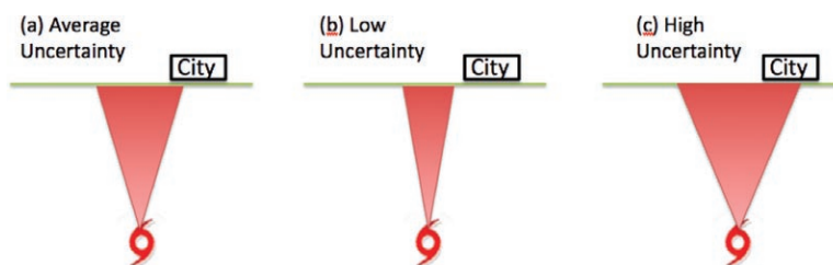
FIG. 1. Conceptual illustration of how situationally dependent uncertainty such as provided by ensembles in track forecasts can improve decision making. (a) The “cone of uncertainty” for a hurricane, estimated using the errors of prior forecasts, provides ambiguous information as to whether to evacuate a city. (b) In this case, a hypothetical calibrated ensemble is suggesting a narrower cone of uncertainty, indicating a decreased threat and implied commensurate actions for the city. (c) Conversely, the uncertainty is much larger and encompasses most of the city, suggesting a potential different course of actions for the city.
