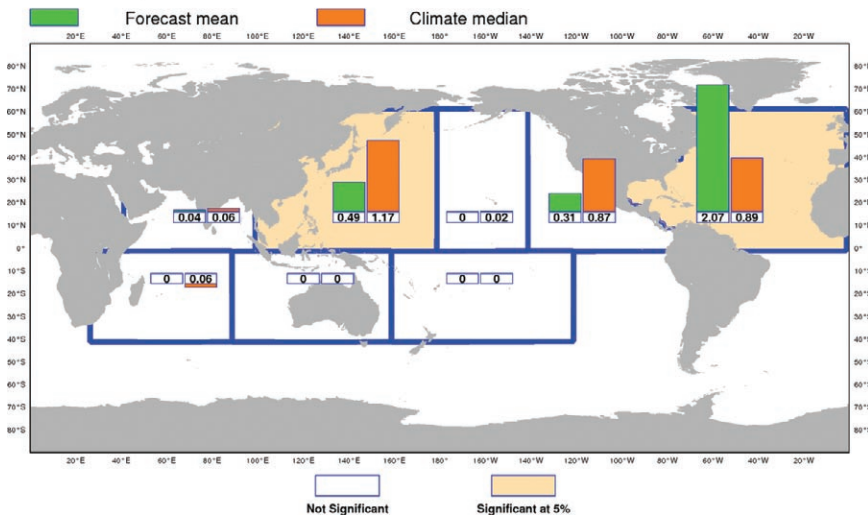
FIG. 4. An example of ECMWF’s extended-range forecast of tropical cyclogenesis, here for the week of 6–12 Sep 2010. Activity is monitored separately in the various basins, separated by the blue lines. The green bars show the mean number of TCs predicted to develop during the week 6–12 Sep (i.e., in each basin count all new TC genes in each ensemble members in that 7-day period and calculate the mean of that number over the ensemble; the actual number is shown below the green bar). The orange bar (and number) is determined from the reforecast climate at this time of the year.
