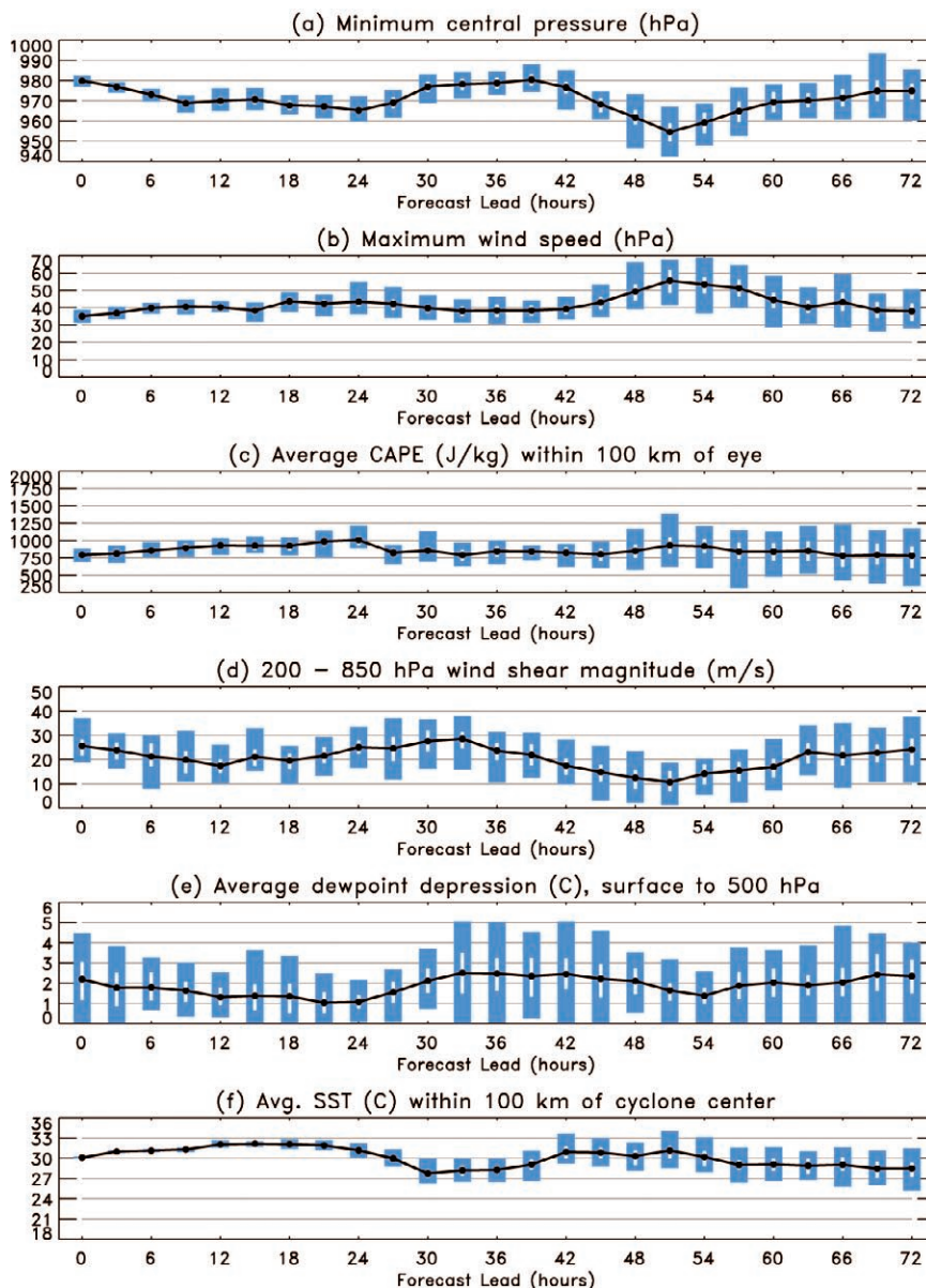
FIG. 3. Synthetic example of a potential meteorogram-style plot of intensity-related information from an ensemble system. Each panel provides the ensemble-mean forecast (solid line and dots), whereas the blue bars denote the lowest and highest values from the ensemble. White lines denote the 20th and 80th percentiles of the distribution.
