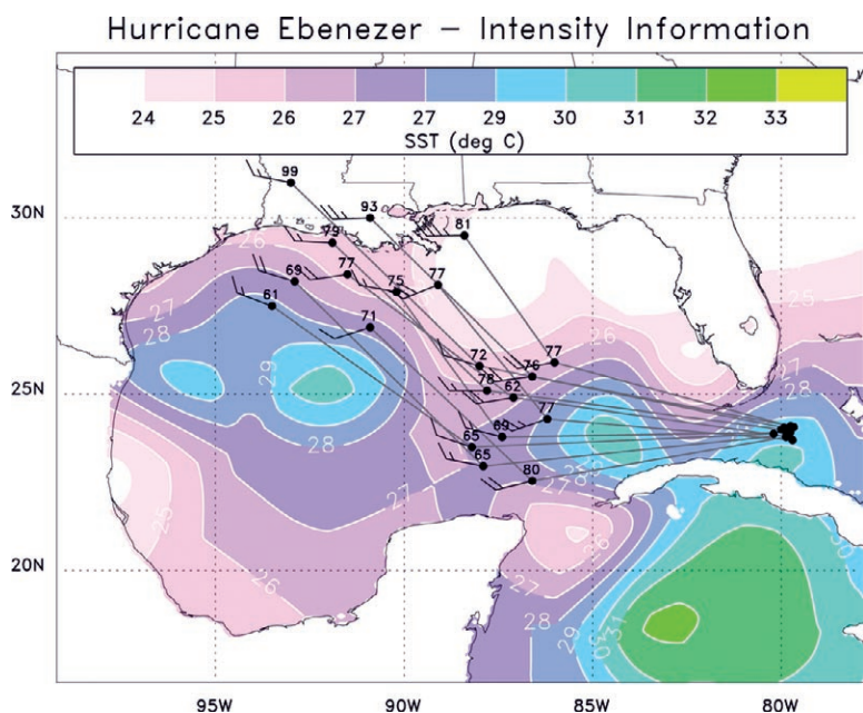
FIG. 2. Illustration of a potential display of intensity-related information. A (synthetic) 10-member ensemble forecast of tracks is shown, with 0-, 24-, and 48-hour positions denoted by the dots. The underlying contours denote the analyzed SST; the wind barbs denote the vertical (200–850 hPa) wind shear, measured in knots (1 kt = 0.5144 \text{ m s}^{-1} ). A full wind barb equals 10 knots, a half barb equals 5 knots. The two numbers plotted over top of the cyclone position denote the model-forecast mean sea level central pressure, measured in hPa minus 900.
