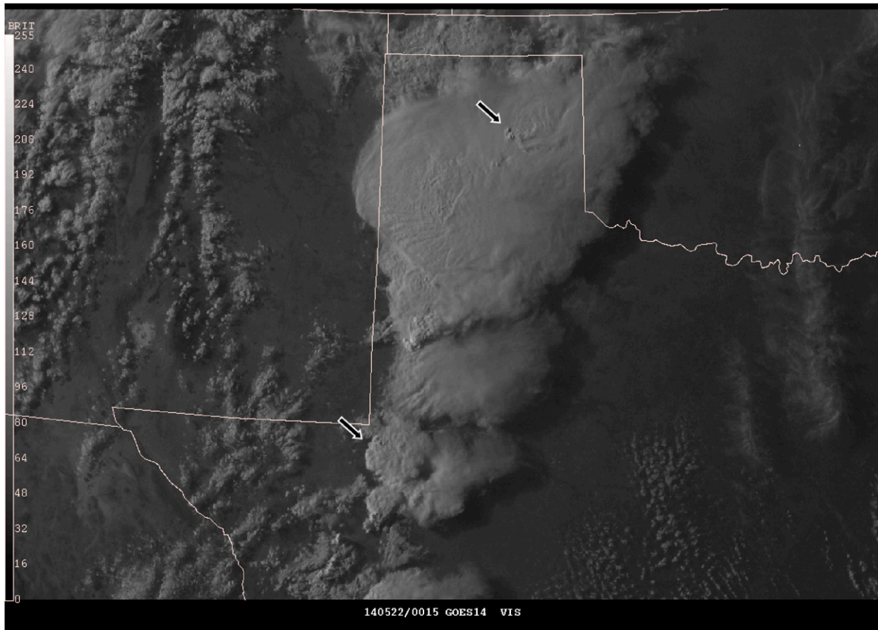
FIG. 3. The 0015 UTC 22 May 2014 GOES-14 visible-channel image. Arrows point to features described in the text. Note the OTs and texturing that are associated with the northern arrow and the new convective development associated with the southern arrow (an animation is available in the online supplemental material: video 3).
