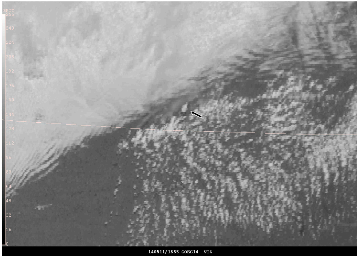
FIG. 2. The 1855 UTC 11 May 2014 GOES-14 visible-channel image. The arrow points to the orphan anvil described in the text. Note the towering Cu just southwest of the orphan anvil where convection would initiate shortly thereafter (an animation is available in the online supplemental material: video 2).
