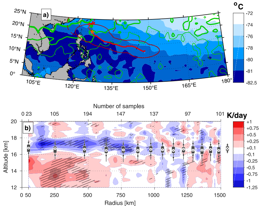
FIG. A1. (a) Average temperature of the cold-point tropopause (shaded; note the spacing of the color scheme) for August–October, weighted by the number of TCs developing each month. The average height of the cold-point tropopause is shown as green isolines (16.6, 16.8, and 17 km, from thin to thick). The average TC track is in red, with the area delimited by a thin red line showing \pm 1 standard deviation from the average track. The star indicates the location of the average lifetime maximum intensity. Best track data collected after maximum intensity are dashed. (b) As in Fig. 4a, but for August–October with the tendency associated with the monthly climatology removed.
