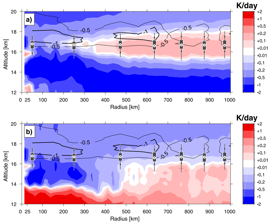
FIG. 6. (a) All-sky, median longwave heating rates and (b) cloudy-sky contribution. The boxplots (tropopause heights) and -0.5 and -1 \text{K day}^{-1} contours (temperature tendencies) are reproduced from Fig. 4a. The sample size is as in Fig. 3.
