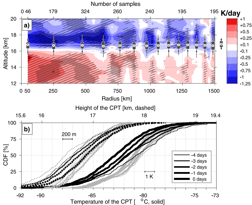
FIG. 4. (a) Temperature tendency ( \text{K day}^{-1} ), defined at each radius and altitude as the slope of the linear regression between the linear temperature and time (relative to maximum intensity). Hatching indicates tendencies for which the coefficient of determination R^2 of the regression exceeds 0.6 in absolute value, and is doubled where R^2 exceeds 0.8. Boxplots show the median height of the tropopause (circled dots) with rectangles showing the interquartile range, whiskers extending from the 1st to the 99th percentiles, and small circles indicating the 10th and 90th percentiles. The white, thin horizontal line emphasizes the median height of the climatological tropopause between 0 and 1500 km (16.9 km), for which statistics are provided in the boxplot outside the main axis. The vertical resolution is 200 m. The horizontal resolution is a function of radius so as to homogenize the sample size between radial bins and is 100 km (30 km) at the 250-km (1500-km) radius. Sample size is linearly interpolated to a regular grid for clarity. (b) Cumulative distribution functions of the height (dashed) and temperature (solid) of the cold-point tropopause (CPT) between 0 and 1000 km, as a function of time relative to the time of maximum intensity (see legend). Black lines show data associated with active TCs, and gray lines show the monthly climatology interpolated onto the location of active TCs.
