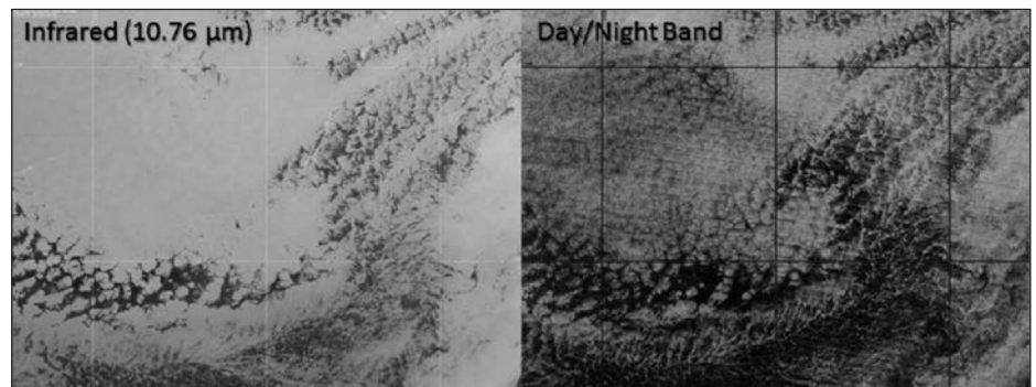
Fig. 2. Cloud scene over the Pacific Ocean from 19 June 2012 under a new moon depicted by (left) infrared and (right) DNB. Figure 2 (right) demonstrates the DNB's ability to utilize reflected nightglow to create detailed imagery.
