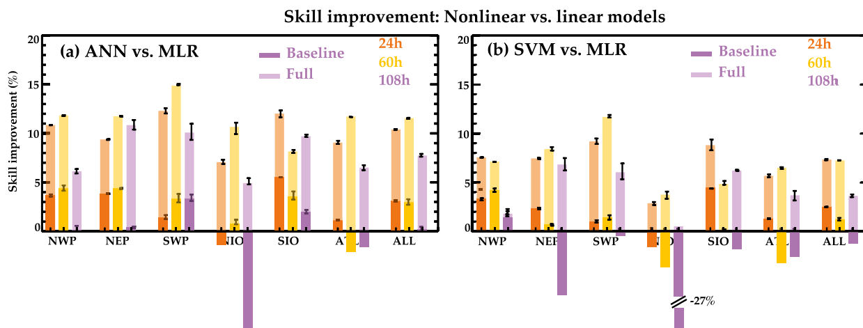
FIG. 4. Percentage of skill improvement for (a) globally trained ANN and (b) SVM relative to regionally trained MLR for baseline models (i.e., only TC initial characteristics, dark color bars) and full models (i.e., including also environmental parameters along the TC track, light color bars) at 24-, 60-, and 108-h lead times, for each basin and globally averaged. Error bars indicate the 95% confidence interval estimated from a bootstrap method.
