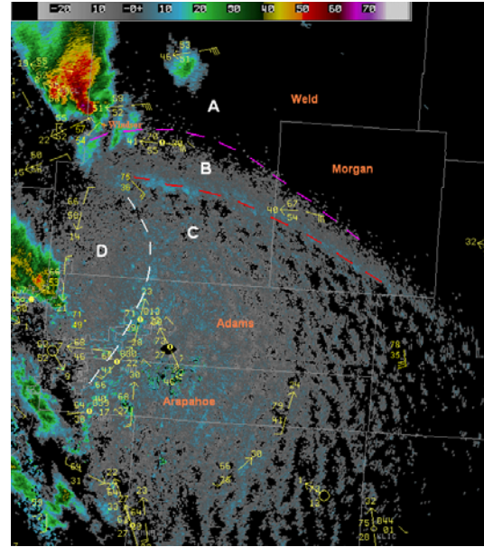
Figure 12. As in Fig. 7, but for 1800 UTC 22 May 2008. Click image to enlarge.
