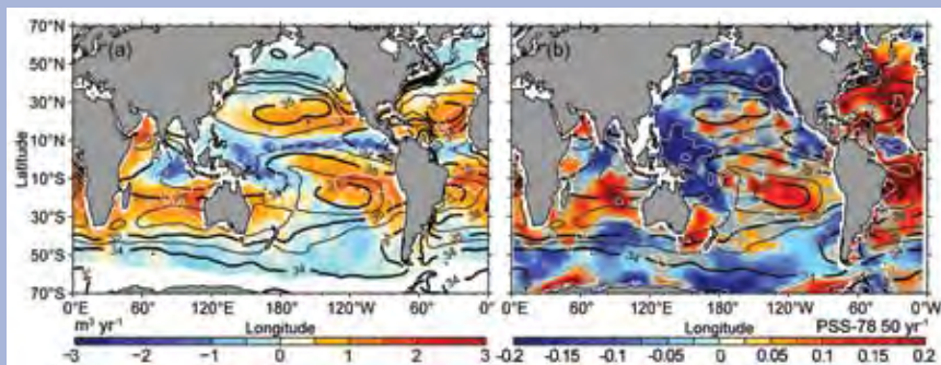
FIG. 3.17. (a) Ocean-atmosphere freshwater flux (E-P; m^3 yr^{-1} ) averaged over 1980–93 (Josey et al. 1998). Contours every 1 m^3 yr^{-1} in white. (b) The 50-year linear surface salinity trend (PSS-78 50 yr^{-1} ). Contours every 0.25 (PSS-78) are plotted in white. On both panels, the 1975 surface mean salinity is contoured black [contour interval 0.5 (PSS-78) for thin lines, 1 for thick lines]. Due to limited observational E-P coverage a direct 1950–2000 climatology is not currently available, however the field produced by Josey et al. 1998 closely matches climatological means developed from many varied products over differing time periods (e.g. da Silva et al. 1994; Schanze et al. 2010) and provide a very similar spatial E-P pattern of correspondence with surface climatological mean salinity. Reproduced from Durack and Wijffels (2010).
