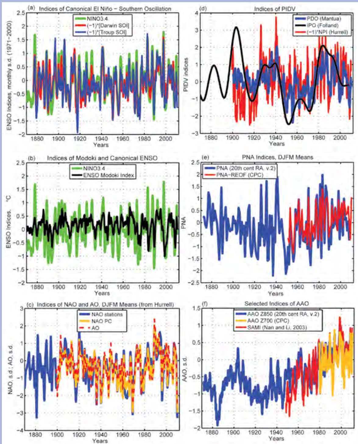
FIG. 1.3. Selected indices of climate variability, as specified in Table 2.3, for the period 1880–2010, grouped into categories: (a) Canonical El Niño–Southern Oscillation (ENSO); (b) the Modoki variant of ENSO; (c) Northern Hemisphere oscillations (NAO, AO, NAM) for the boreal cold season; (d) indices of Pacific Interdecadal Variability; (e) Pacific–North American indices for the boreal cold season; (f) Southern
