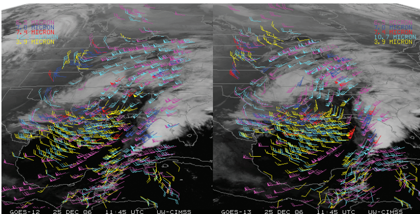
FIG. 4. GOES-12 (left) and GOES-13 (right) atmospheric motion vectors (AMVs) for 25 December 2006 plotted over band-4 (10.7 \mu\text{m} ) images. The color coding differentiates the satellite bands used in AMV derivation. Note that the viewing angles are different. Also, not all AMVs are shown for clarity of display. (Figure courtesy of D. Stettner.)
