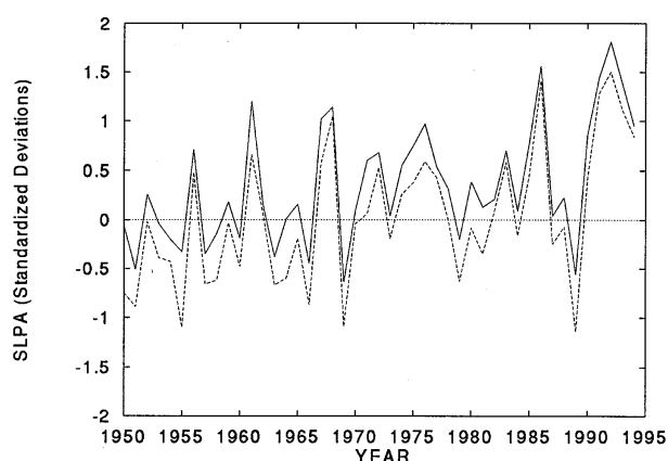
FIG. 12. Time series of the JAS SLP index (dashed) in the TA along with a corrected SLP index (solid) created by removing the effect of tropical storms and hurricanes.
