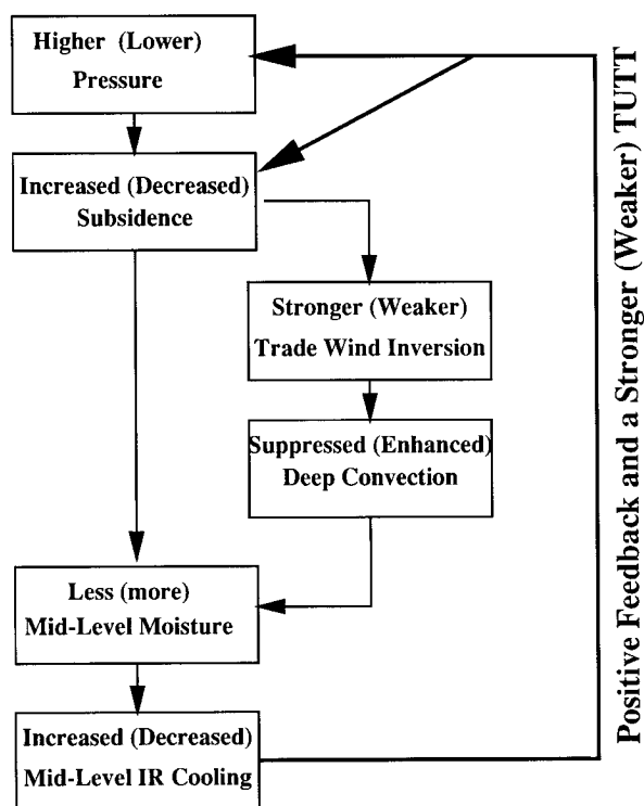
FIG. 16. Flow chart depicting the major elements of the hypothesized positive feedback loop between SLP pressure, midlevel moisture and convection and IR cooling to space. During periods of anomalously high (low) surface pressure, subsidence is increased (decreased). This change in the rate of sinking acts twofold to reduce (increase) midlevel moisture while at the same time decreasing (increasing) deep convective activity. The combination of larger (smaller) moisture gradients in the vertical and the decrease (increase) in convective activity result in more (less) IR cooling to space. This increase (decrease) in cooling acts to reinforce the high (low) pressure condition.
