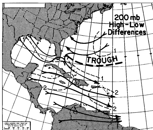
FIG. 3. Composite differences of the 200-mb wind field during July through September for periods of high pressure minus periods of low pressure in the tropical Atlantic. Isotachs are drawn every \text{m s}^{-1} .
