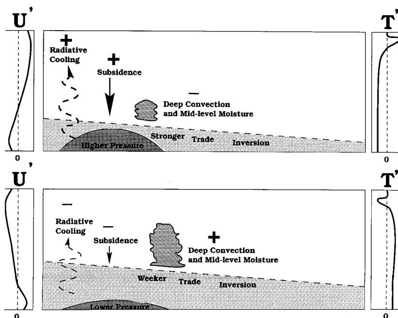
FIG. 15. Idealized schematic of the conditions characteristic of anomalously higher pressure (top) and anomalously lower pressure conditions (bottom) in the the tropical Atlantic. When pressures are anomalously high (low), increased subsidence (decreased) has the effect of reducing (increasing) midlevel moisture and strengthening (weakening) the trade wind inversion. The combined effects of relative reduction (increase) of convection and midlevel moisture enhances (suppresses) IR cooling to space. This anomalous cooling (warming) of the midlevels enhances upper-level westerly (easterly) and lower-level easterly (westerly) zonal wind anomalies.
