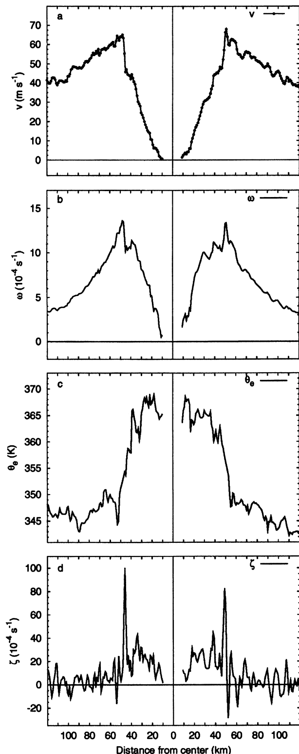
FIG. 6. Cross sections of (a) tangential wind, (b) angular velocity, (c) \theta_e , and (d) vorticity calculated from flight-level (10 000 ft) reconnaissance data of Hurricane Luis for 2230–2308 UTC 3 Sep 1995.
