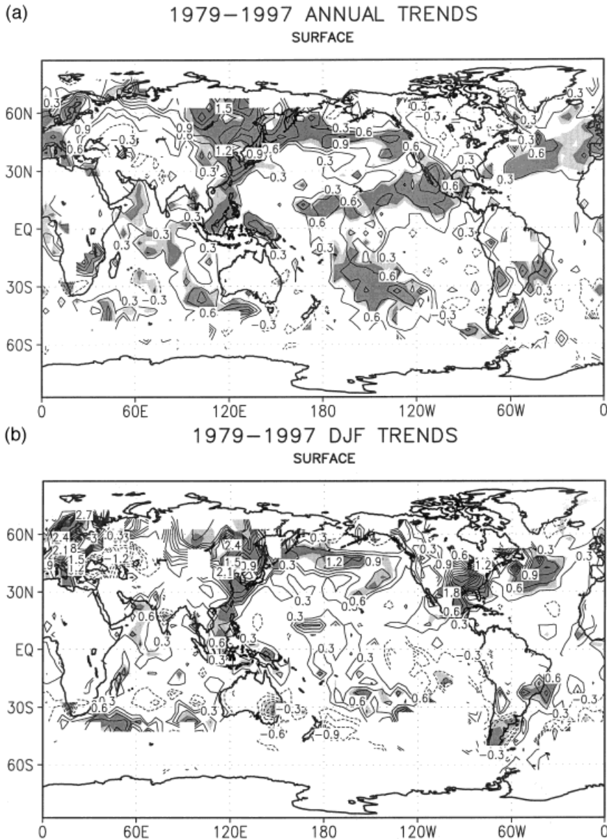
Figure 4. As in Figure 1, but for the surface observational network. Regions not contoured indicate no available data
