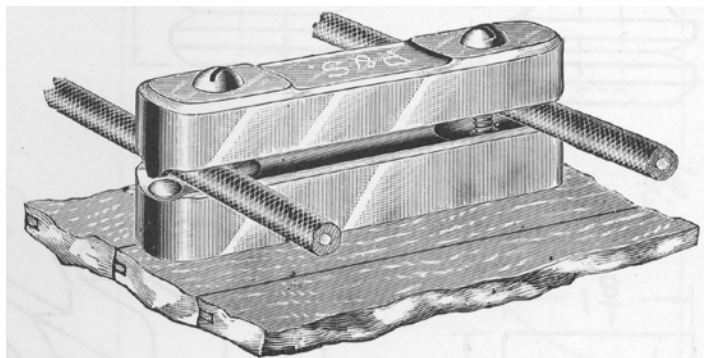
Figure 8. Illustration of cleat with wires in use (Tod 1977:28).
