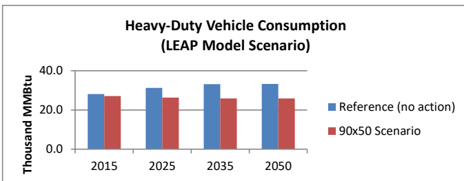
Figure 5.8: LEAP model scenario for Heavy-duty vehicle energy consumption over the benchmark years.
