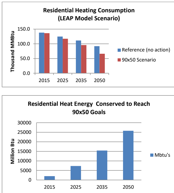
Figure 7.5: LEAP model scenario of residential heat consumption over the benchmark years.
