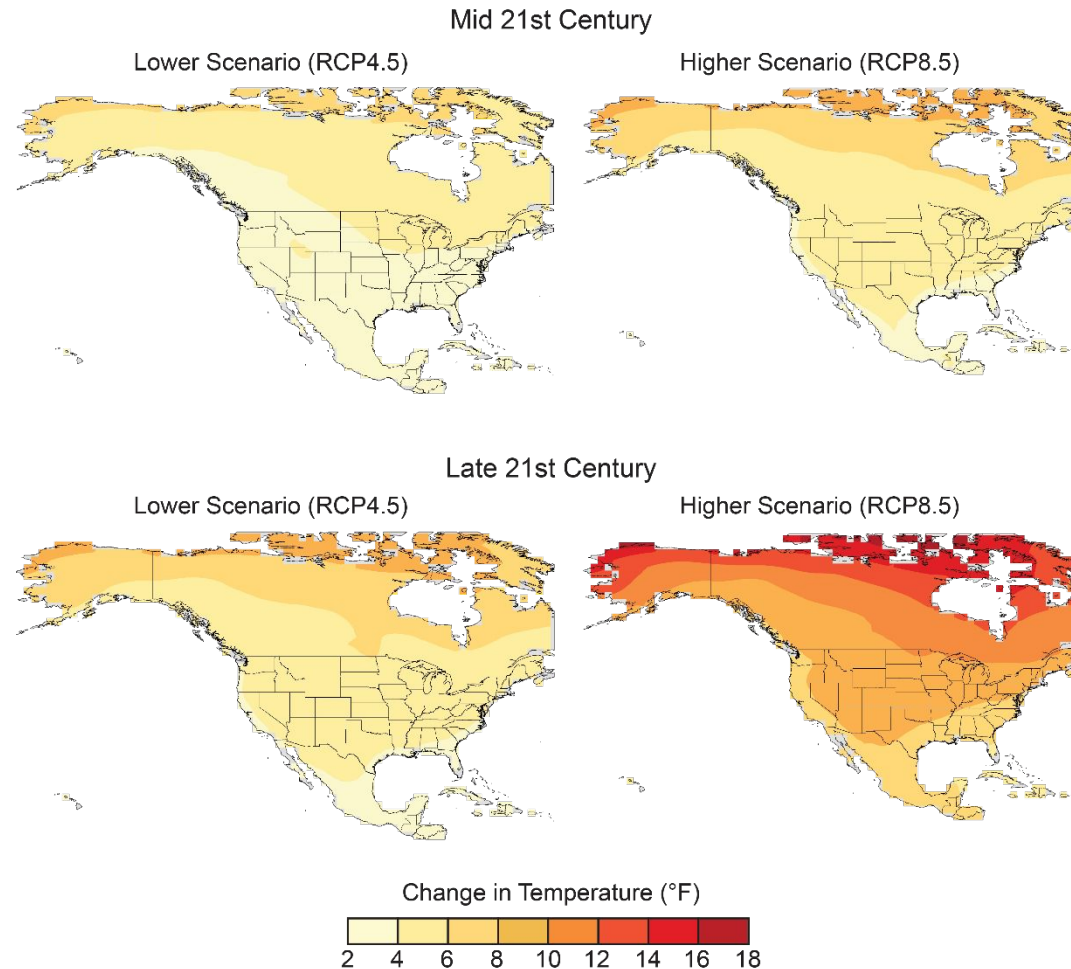
Projected Changes in Annual Average Temperature
