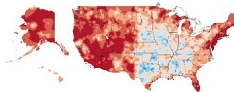
Summer Temperature
