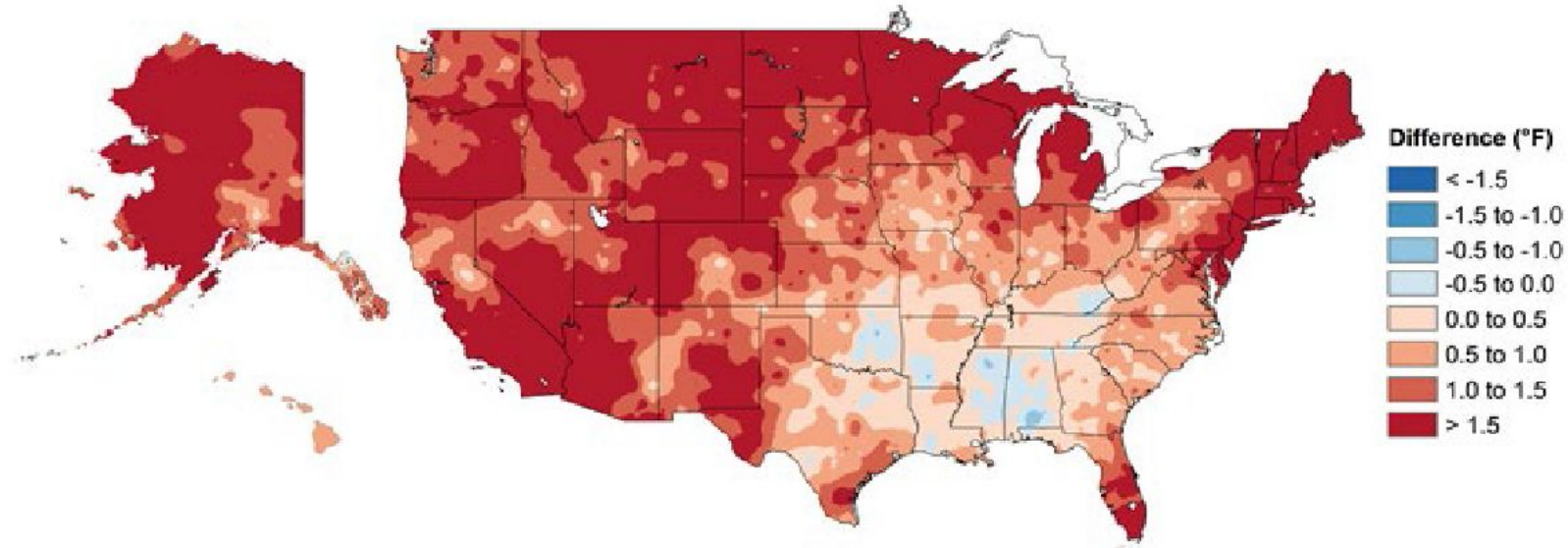
Annual Temperature
