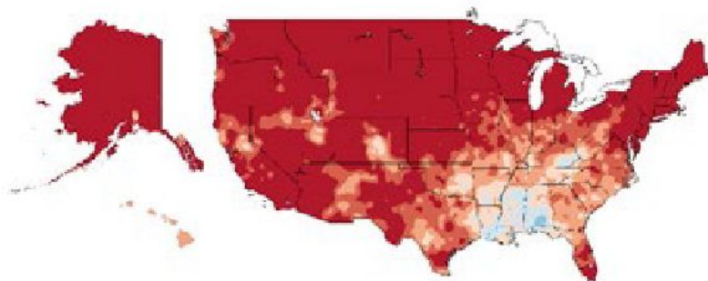
Winter Temperature
