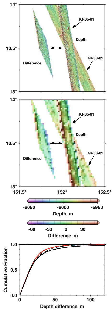
Fig. 1 Overlapping multibeam swaths KR05-01 and MR06-01 and their differences in depth where they intersect (the parallelogram-shaped areas) are plotted on a 6 arc-second grid (top panel), and the same but plotted as median depths on a 1-min Mercator grid (middle panel). A cumulative histogram (bottom panel) plots depth differences between KR05-01 and MR06-01 (red line), and between KR05-01 and combined MR06-01, MR99-K06, and MR00-K02 overlaps. The solid black line is from differences using a 6 arc-second grid, and the dashed line is the same from a 1 min grid
