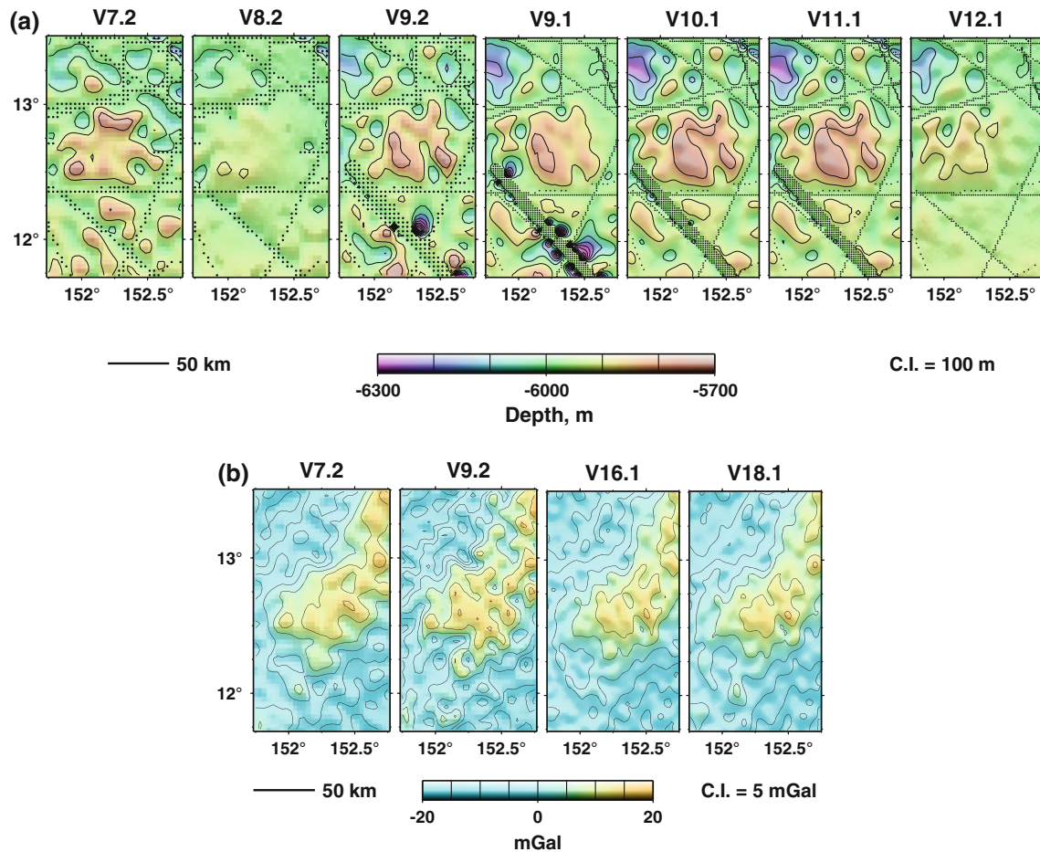
Fig. 5 a Bathymetric model versions and b satellite-derived gravity anomalies over smooth seafloor (Table 1 links gravity to bathymetry versions). Black dots are grid cells constrained by ship soundings. Short-wavelength gravity anomalies incorrectly give rise to corresponding
