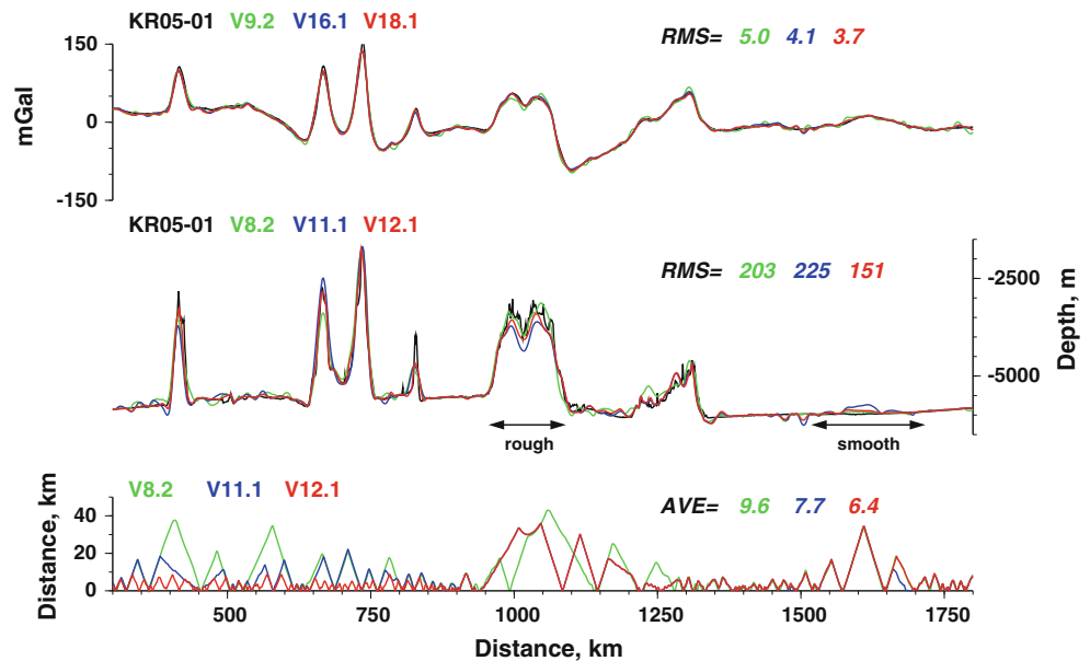
Fig. 3 Gravity ( top ), bathymetry ( middle ), and distance to nearest bathymetry control point ( bottom ) profiles along the track of ship survey KR05-01, comparing values measured by the ship with estimates from various altimetry models, indicated by colored lines and labels. RMS numbers are root-mean-square differences between altimetry model estimates and KR05-01 measurements. The areas labeled “smooth” and “rough” are examined in more detail in Figs. 6 and 9
