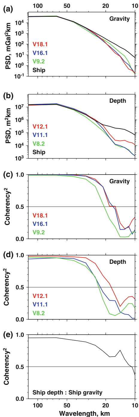
Fig. 4 Power spectral density (PSD) and cross-spectral coherency from the portion of the profiles shown in Fig. 3 that runs from 350 to 1,400 km. a Gravity PSD, b depth PSD, c gravity coherency, d depth coherency, and e coherency between gravity and depth as both are measured by KR05-01
