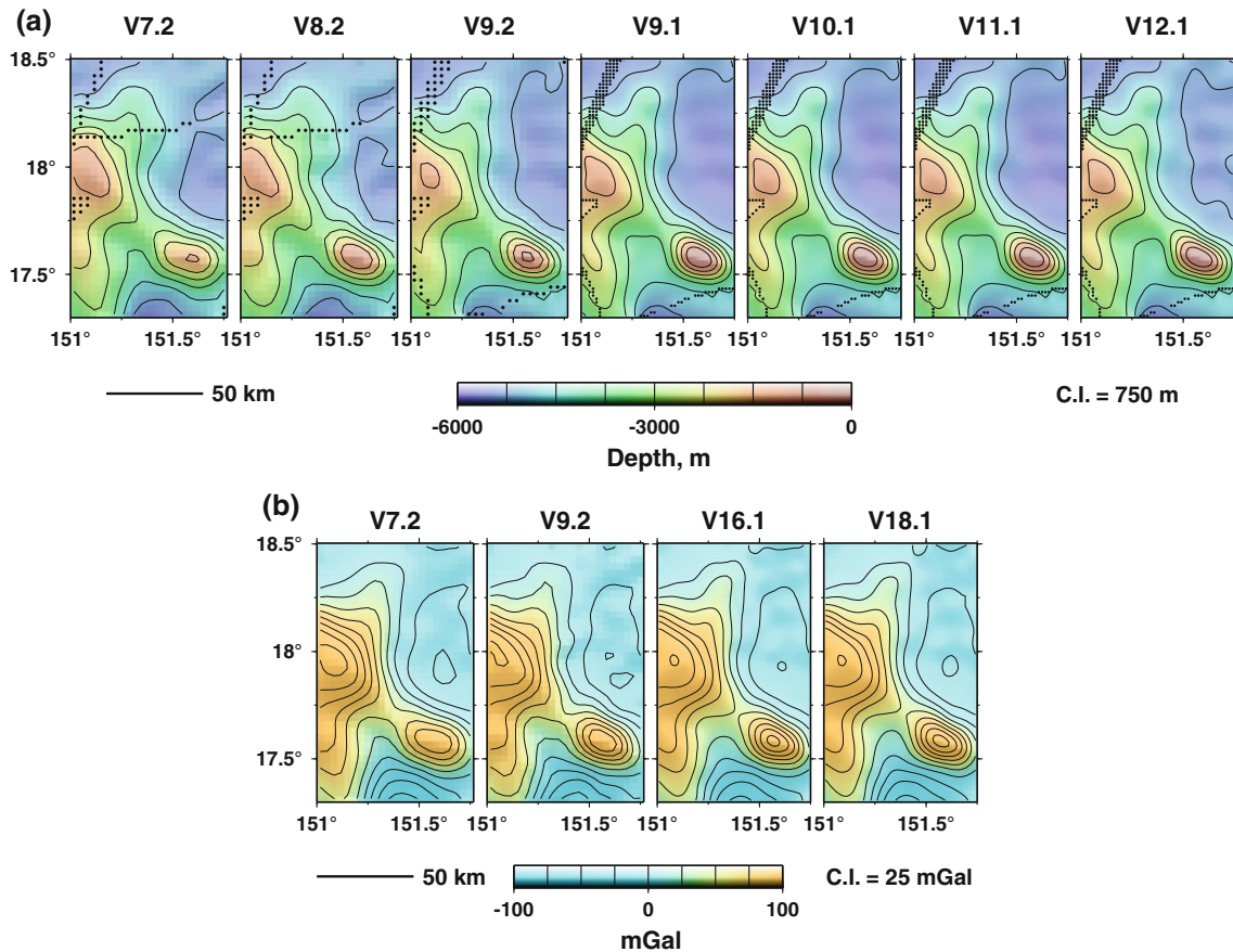
Fig. 8 a Bathymetric model versions and b satellite-derived gravity over rough seafloor. Table reference and black dots are the same as in Fig. 5 caption. Prediction-band (15–160 km) gravity anomalies are correctly passed into the bathymetry models
