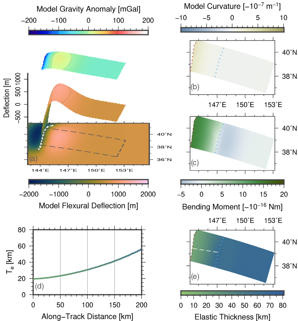
Figure 8. For a region offshore NE Japan (ID:JP02) and using the W lithosphere rheology, a map of the original model output for the deflection w and a 3-D visualization of the best-fitting flexural surface selected are shown in (a). Also displayed in (a) is the expected marine gravity anomaly \Delta g as calculated from w . The contours are drawn every 1000 m for w and every 200 mGal for \Delta g . From w , the curvature as seen in (b) is computed. The red dotted line marks the locations of the largest magnitudes of the curvature at the trench outer slope, while the blue dotted line traces the smallest magnitudes of the curvature just seawards of the outer rise. In turn, the curvature is used to compute the bending moment as seen in (c). The elastic thickness values T_e are then obtained from the moment–curvature relation which is specific to the W set of models. Subfigure (d) shows a trench-perpendicular profile of T_e , the location of which is shown in relation to the model region mapped in subfigure (e).
