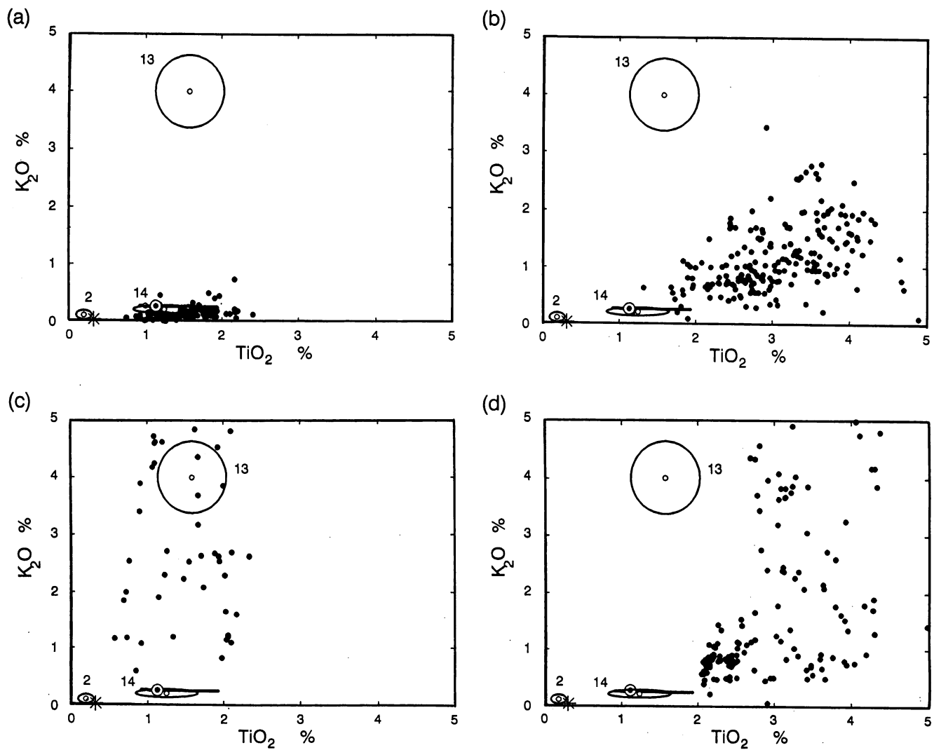
Fig. 5. K_2O as a function of TiO_2 for the same magmas as in Figure 4. The ellipses correspond to one standard deviation. The magmas plotted in Figures 5a-5d are the same as those in Figures 4a-4d.
