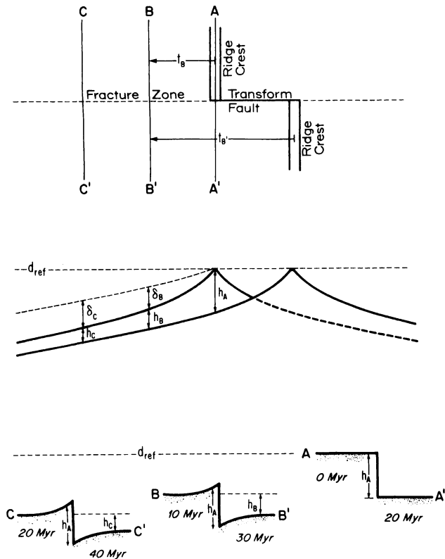
Fig. 1. Evolution of a fracture zone. (Top) Spreading ridges offset by a transform fault. The age offset across the FZ is t_{B'} - t_B . (Center) The h 's are the differences in ocean floor depth between locations far to either side of the FZ. The initial height of the scarp at the FZ is h_A . If the FZ does not slip, the scarp height must remain constant. The constancy of scarp height and the decrease in h with age cause the lithosphere in the vicinity of the FZ to bend. The flexural amplitude \delta_B is the difference between h_A and h_B . Similarly, \delta_C = h_A - h_C . (Bottom) Sketch of bathymetry along profiles A-A', B-B', and C-C' illustrating the lithospheric flexure described above.
