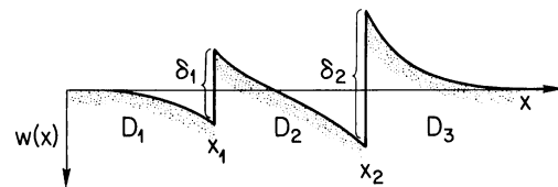
Fig. 5. Model used to calculate the flexural topography w(x) across multiple FZ's. Two FZ's are located at x_1 and x_2 and have flexural amplitudes \delta_1 and \delta_2 . The flexural rigidity is different for each segment of lithosphere.
