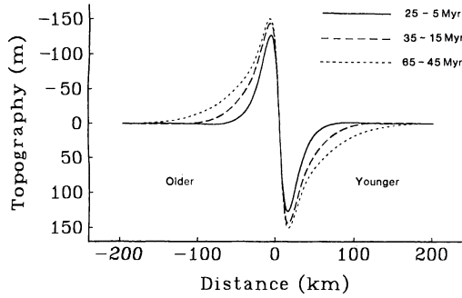
Fig. 9. Flexural topography associated with heat conduction across a FZ with a 20-Myr age offset. Ages of younger side are 5 Myr (solid line), 15 Myr (dashed line), and 45 Myr (dotted line). This topography broadens with age as heat diffuses across the FZ. The amplitude of this effect has been overestimated, especially on the older side of the FZ, since we used the flexural rigidity-age relation (8) of the younger side of the FZ in the theoretical calculation.
