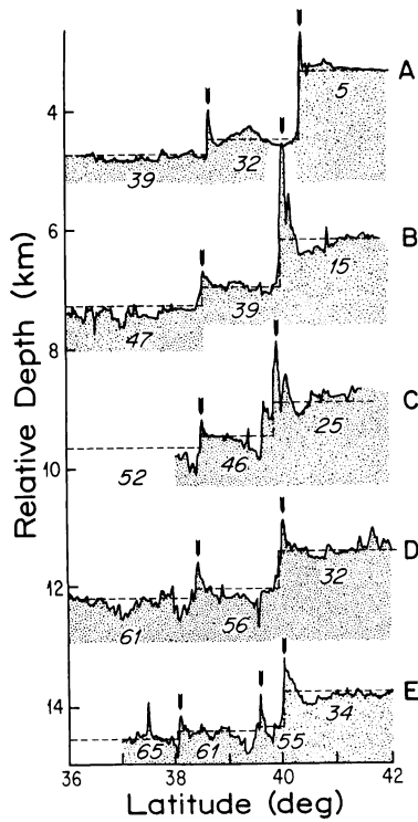
Fig. 3. Relative depth as a function of latitude along profiles A-E. Profiles are offset in increments of 2.3 km. Dashed lines are depths predicted from (1). FZ's are marked by arrows. The Pioneer FZ appears on each profile at 38°-39°N. The Mendocino FZ lies at ~40°N. The Mendocino S. is well defined on profile E at 39.6°N. It is seen that (1) predicts the overall change in depth across a FZ but not the scarp height.
