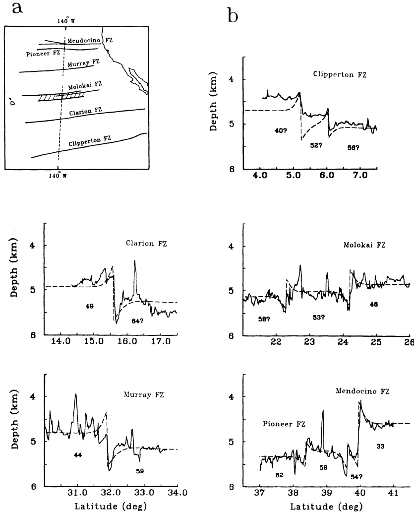
Fig. 8. (a) Location map (gnomonic projection) of major North Pacific fracture zones. Dashed lines indicate ship tracks. (b) Comparison of flexure model (dashed curve) with bathymetry across each of the major FZ's. Question marks indicate that ages are based upon the depth-age relation.
