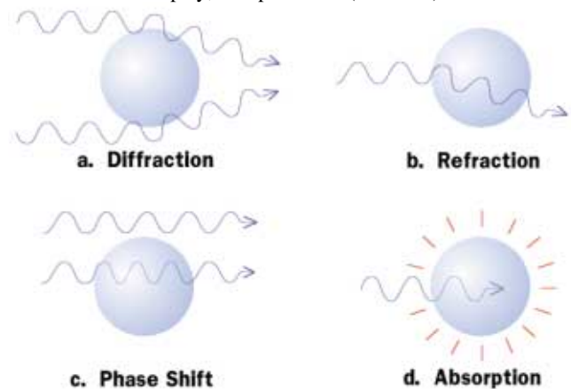
Fig. 2.1 Large particle light scattering and absorption. Diffraction (a) and refraction (b) combine to “bend” light to “fill in the shadow” behind the particle. Diffraction, an edge effect, causes photons passing very close to a particle to bend into the shadow area; refraction is a result of the light wavefront slowing down as it enters the particle. While the photon is within the particle, its wavelength is also shortened. Thus, when it emerges from the particle, it may vibrate out of phase with adjacent photons and interfere with their ability to propagate in a pre-prescribed direction. This effect (phase shift) is shown in (c). As a fourth possibility, the photon may be absorbed by the particle (d). In this case, the internal energy of the particle is increased. The particle may rotate faster or its molecules may vibrate with greater amplitude.
