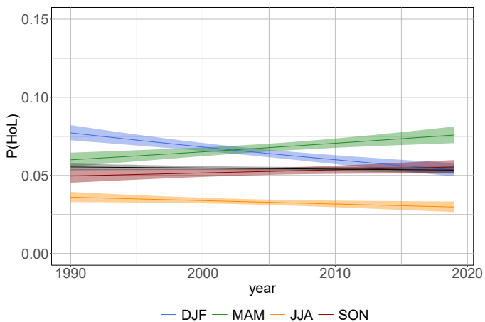
(a) High-over-Low blocking, 40^\circ W to 30^\circ E
