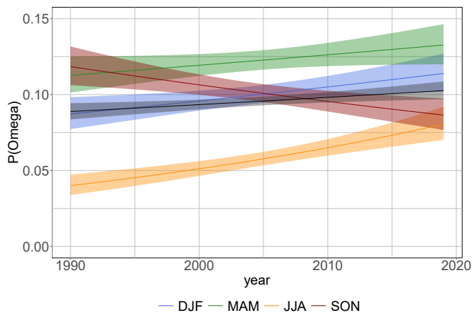
(b) Omega blocking, 40^\circ W to 30^\circ E
