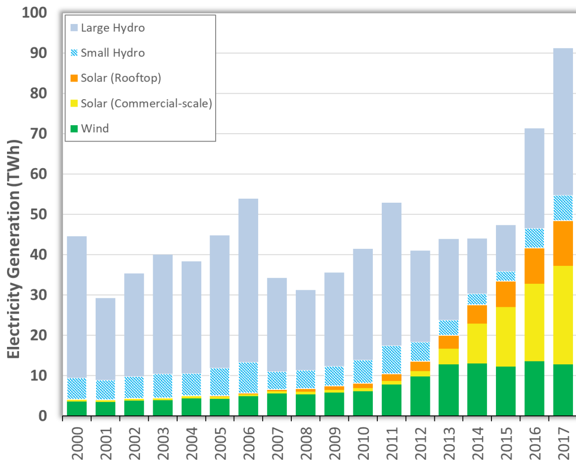
Figure 10. In-State Hydro, Solar, and Wind Electricity Generation. This figure shows the amounts of electricity generated by California’s in-state wind power projects, large commercial-scale solar power projects, rooftop solar panels, and hydropower generation stations. The unit is in terawatt-hour (1 TWh = 10 9 kWh).
