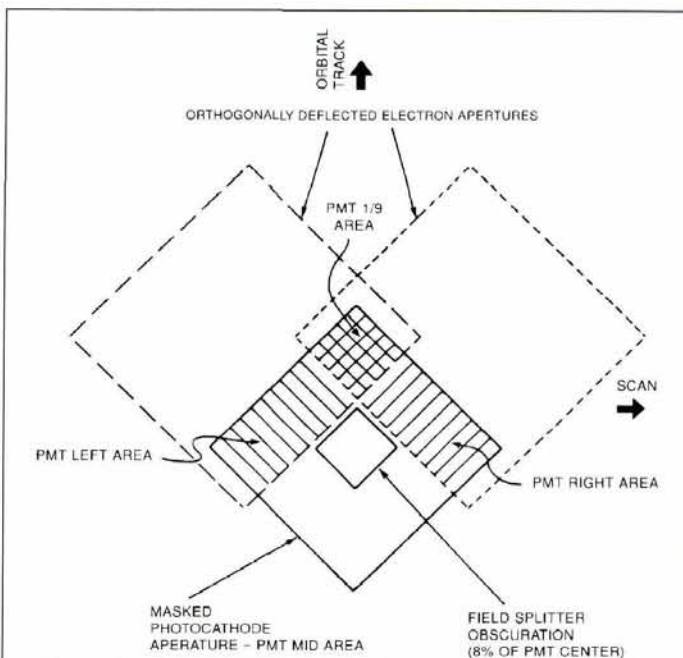
Figure 4. Aperture switching of the DMSP-OLS photomultiplier tube (PMT). The switching reduces the size of the detector image on the Earth's surface during the first and last quarter of each scanline. Figure courtesy of Westinghouse Electric Corporation.
