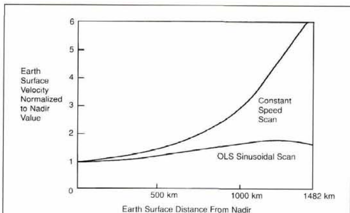
Figure 3. Uniformity of the DMSP-OLS Earth surface scan velocity. Figure courtesy of Westinghouse Electric Corporation.
