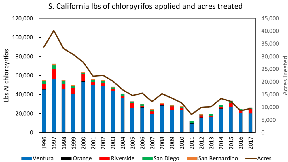
Figure 10. Foliar treatments of chlorpyrifos in citrus: southern California, 1996-2017, pounds AI applied and acres treated
