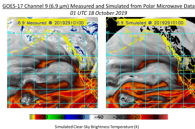
Figure 6: Measured (left) and cloud-free simulated (right) GOES-17 6.9 \mu\text{m} water vapor imagery from 01 UTC 18 October 2019. Black areas in the simulated imagery are missing due to precipitation or high zenith angle.
