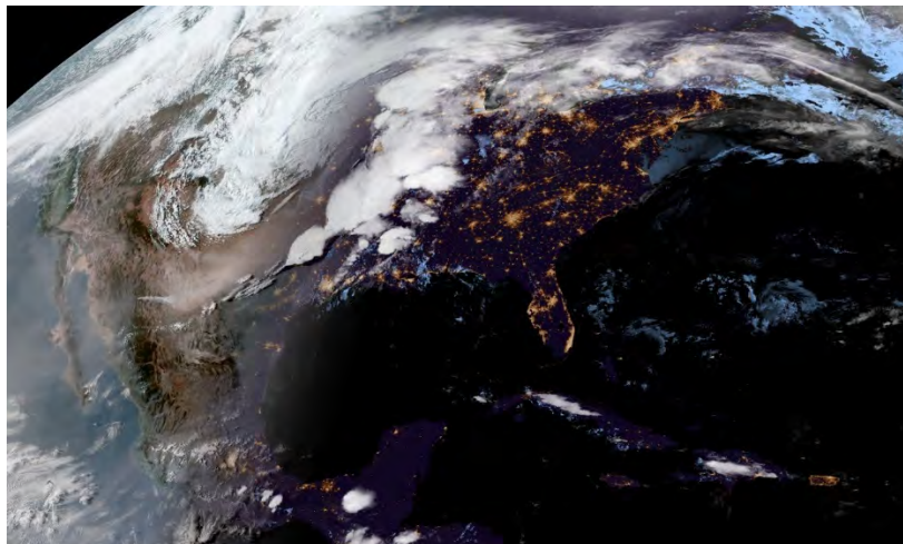
Figure 1: Figure: GOES-16 ABI GeoColor imagery from 14 April 2018 at 0002Z depicts a powerful Springtime midlatitude cyclone with pre-frontal severe thunderstorms over the central U.S., with lofted dust over Texas, a biomass smoke plume over north/central Mexico. Meanwhile, the eastern U.S. enjoys relatively quiescent conditions as city lights shine under the clear, early evening skies.
