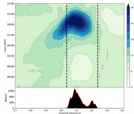
Figure 1. Composite diurnal cycle based on CMORPH precipitation in boreal summer averaged latitudinally across Luzon, with average topography from NOAA ETOPO2 in the same cross section shown below the plot. The average longitudes of the shoreline are denoted as dotted black vertical lines.
