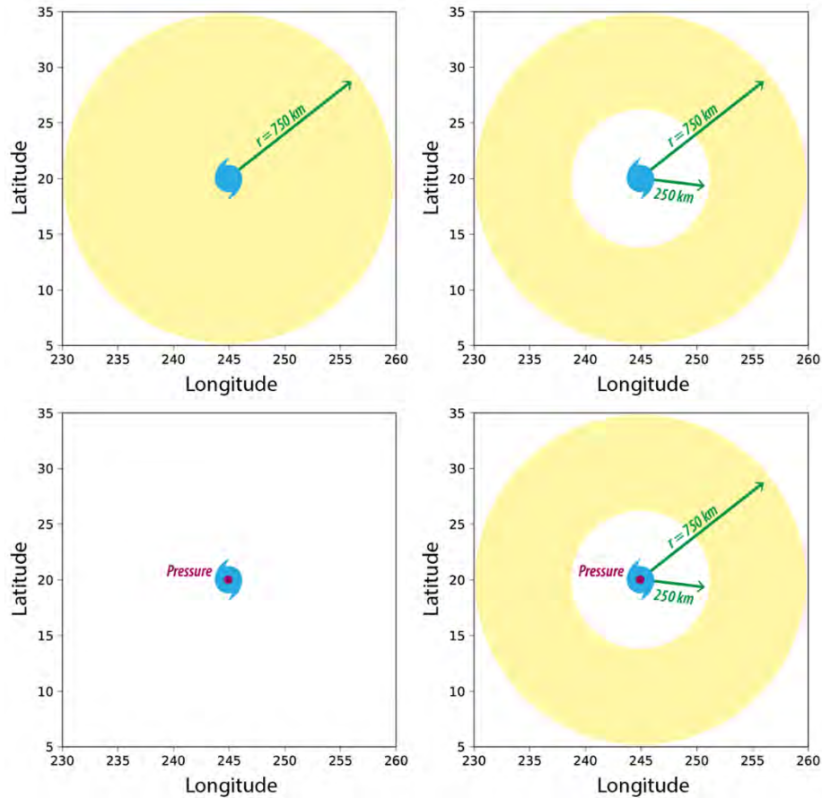
Figure 1. Schematic for experimental design for testing TC vortex initialization with MTCSWA in HRRF.
