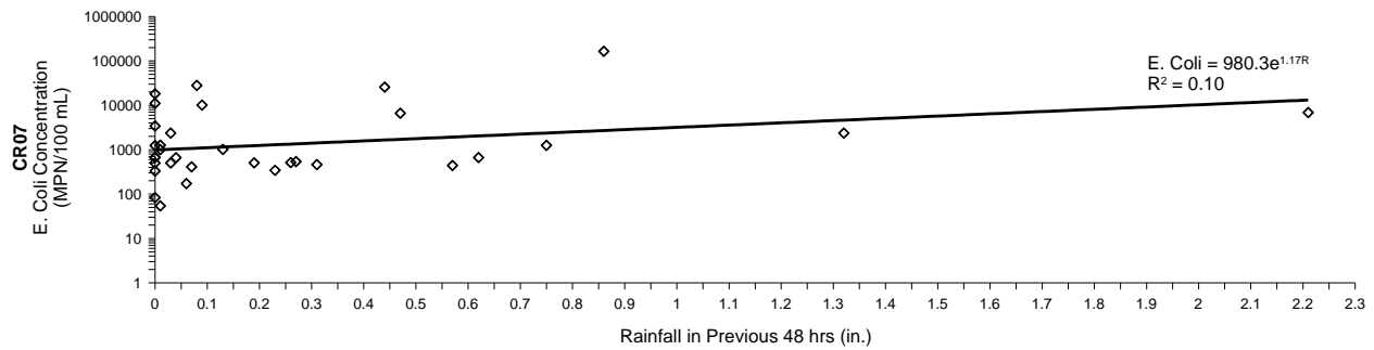
Figure 105. E. coli concentration response to 48-hour prior total rainfall for CR07
