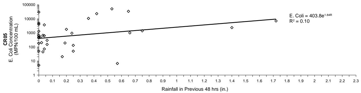
Figure 92. E. coli concentration response to 48-hour prior total rainfall for CR05
