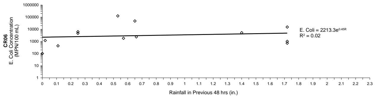
Figure 94. E. coli concentration response to 48-hour prior total rainfall for CR06
