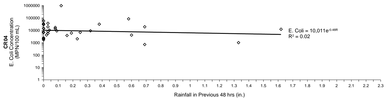
Figure 93. E. coli concentration response to 48-hour prior total rainfall for CR04
