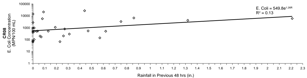
Figure 106. E. coli concentration response to 48-hour prior total rainfall for CR08
