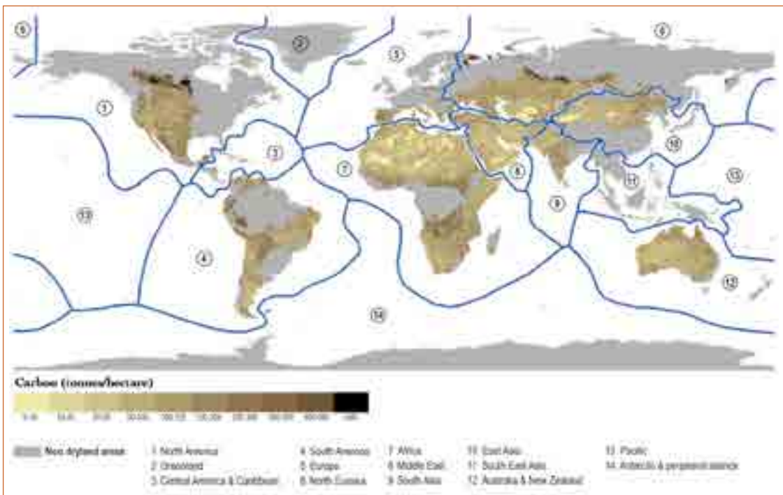
Figure 11 · Carbon mass per hectare throughout the drylands.
