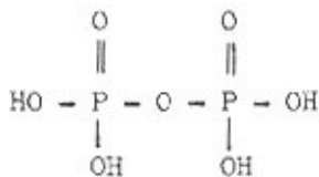
Pyrophosphoric acid
