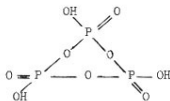
Cyclic form
