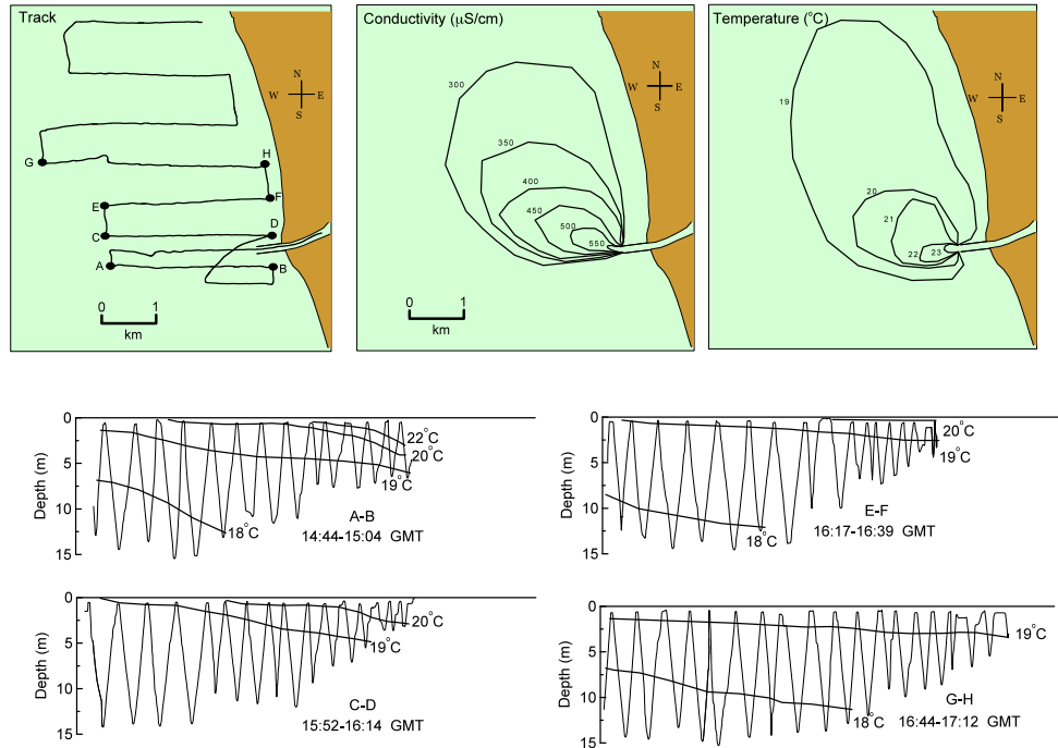
Figure 3.12 CTD survey map and selected temperature transects on June 22, 2006.
