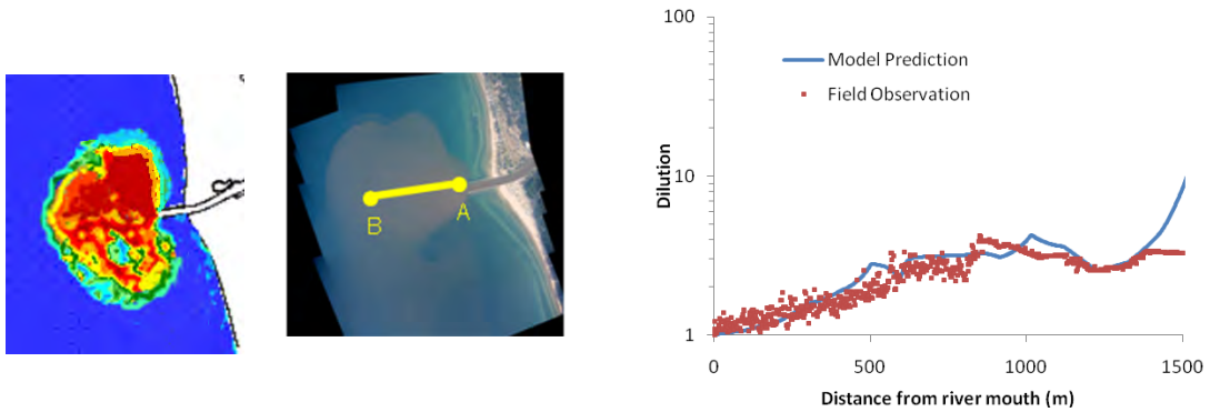
Figure 6.4 Comparison of PARTIC3D predicted and observed dilution on June 6, 2007.
