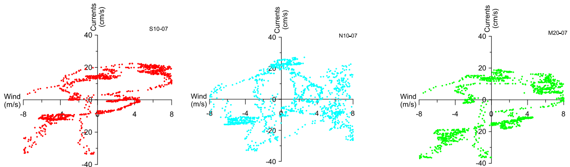
c) Longshore surface current and wind scatter
