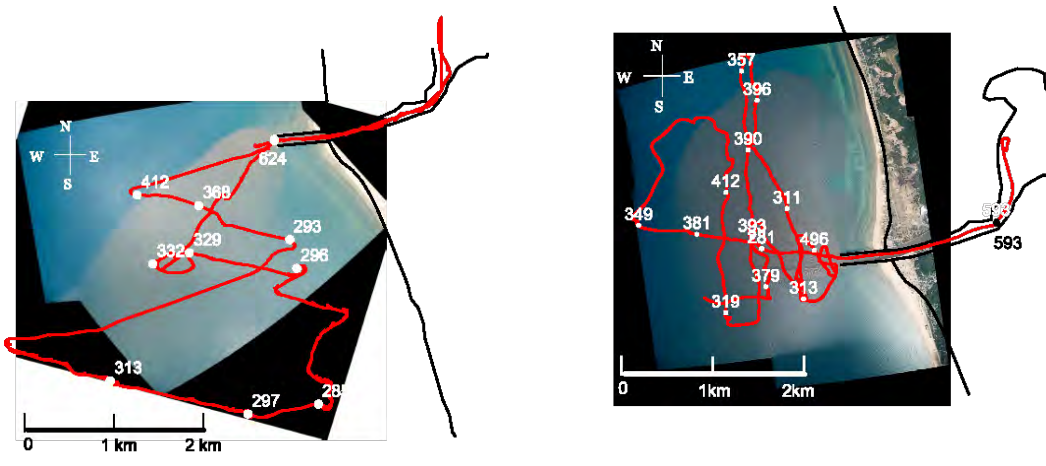
c) Surface conductivity in \mu\text{S}/\text{cm} on June 5 (right), and 6 (left), 2007.
