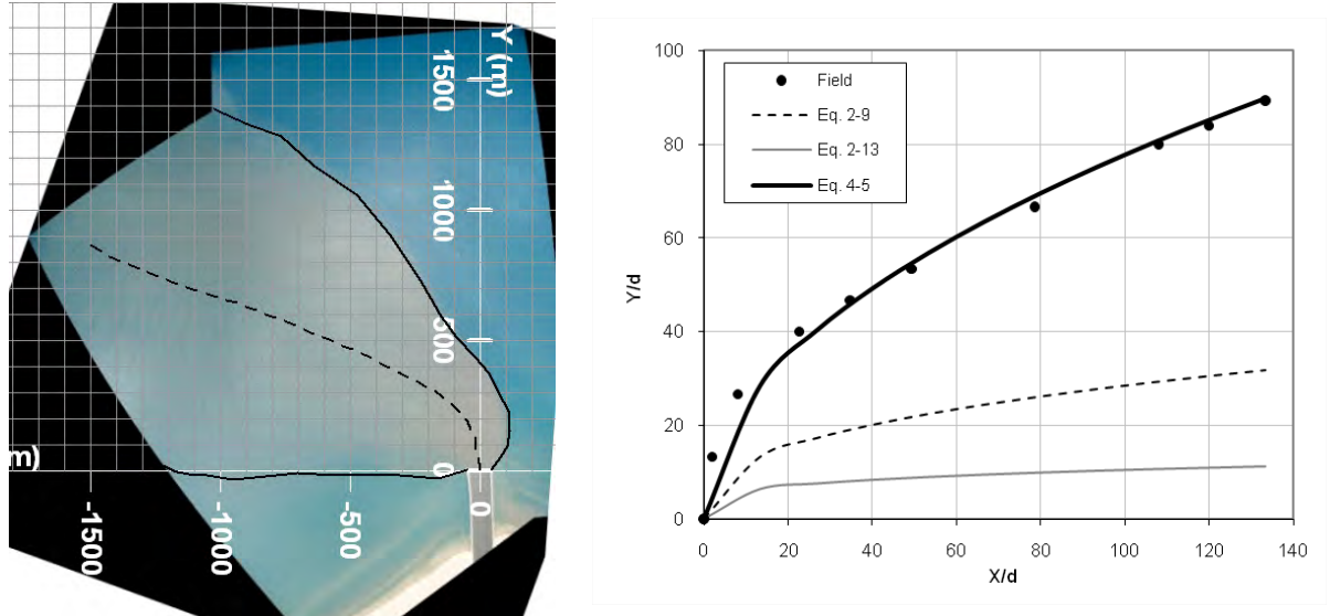
Figure 4.12 An unattached jet trajectory overlaid on the aerial photo on June 5, 2007 16:55 GMT (left); and comparison of predicted and observed jet trajectory (right).
