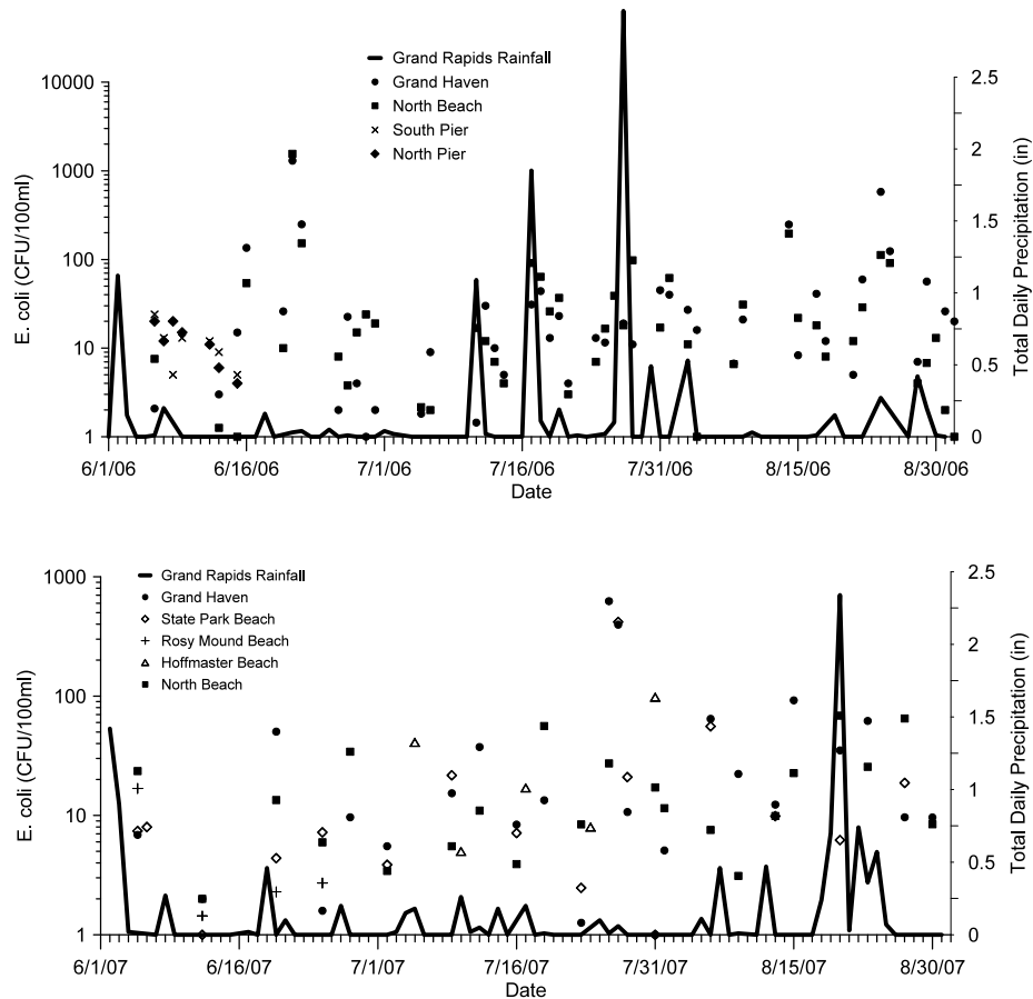
Figure 4.16 Beach bacterial samples and total daily precipitation at selected beach sites during May-August 2006 (top) and 2007 (bottom).
