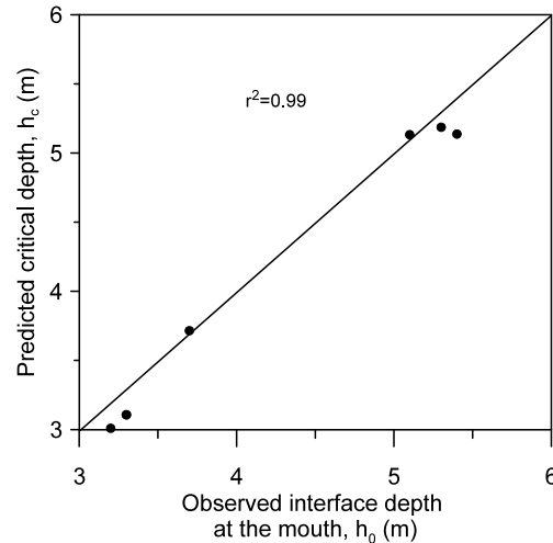
Figure 4.7 Predicted critical depth, h_c versus observed interface depth at the mouth, h_0 .
