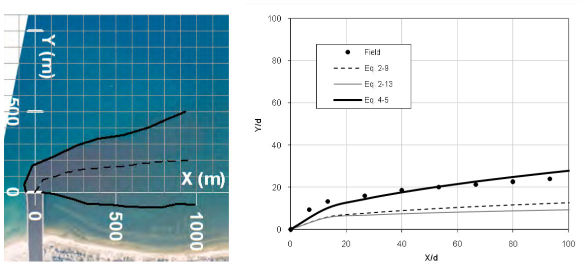
Figure 4.11 A shore attached jet trajectory overlaid on the aerial photo on July 18, 2007 13:15 GMT (left); and comparison of predicted and observed jet trajectory (right).
