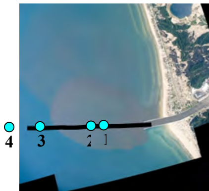
Figure 5.15 Model temperature versus field data on August 22, 2006.
