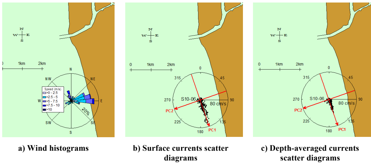
Figure 3.15 Polar wind and currents diagrams at S10-06 from August 7 to 11, 2006.
