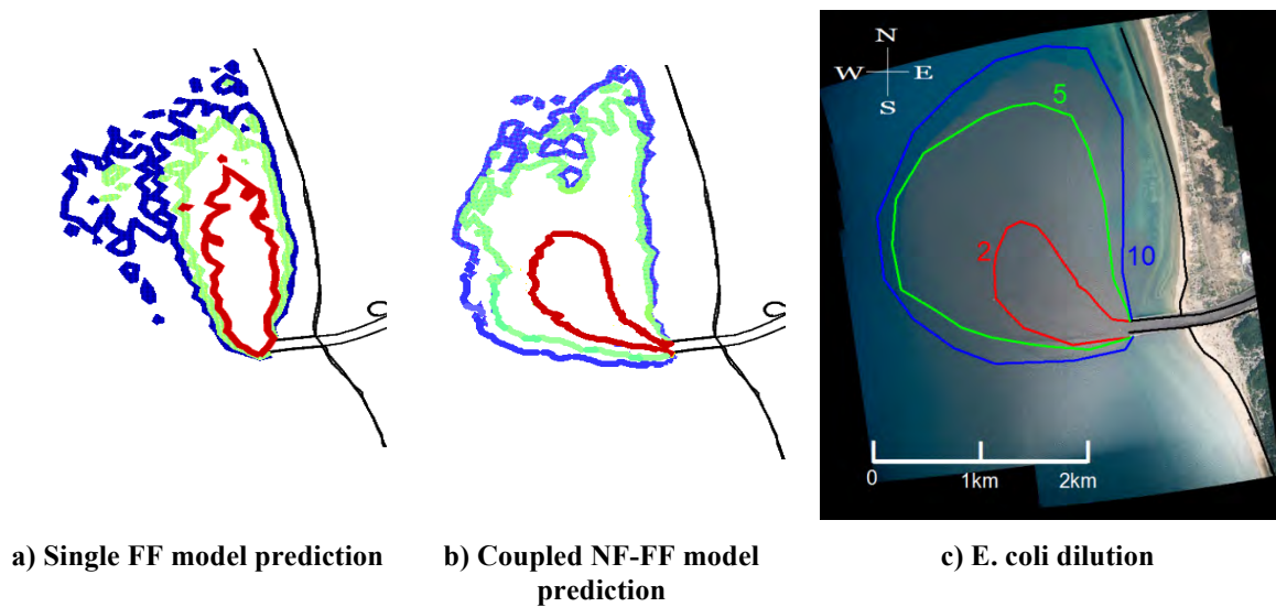
Figure 6.7 Comparison of E. coli dilution contours (red 2:1, green 5:1, and blue 10:1) with the single FF and coupled NF-FF model predictions on June 6, 2007.
