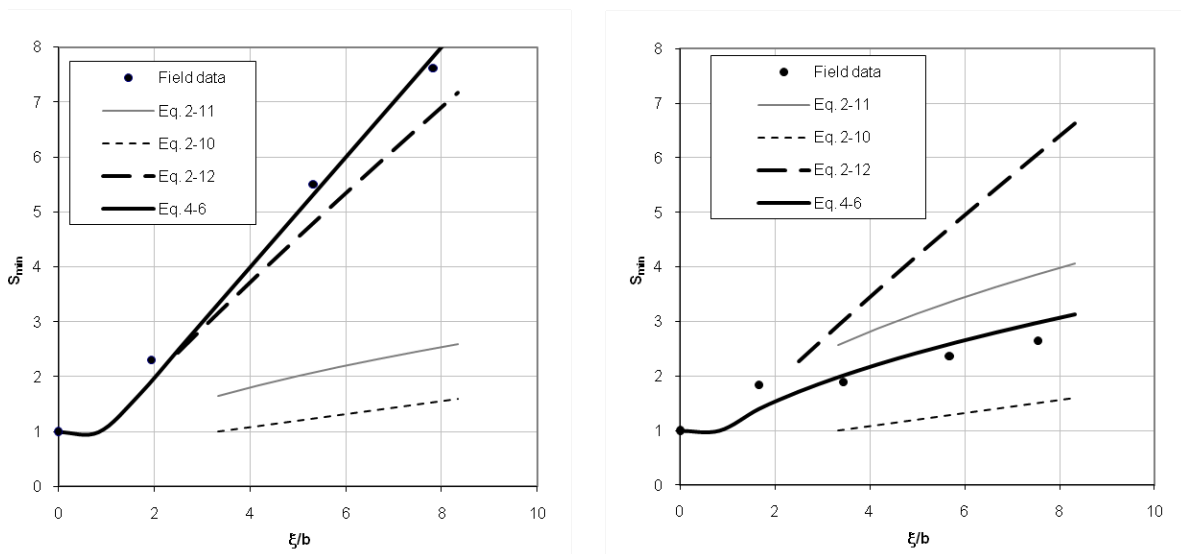
Figure 4.13 Comparison of predicted and observed minimum dilutions of an attached plume on July 18, 2007 13:15 GMT (left), and an unattached plume on June 5, 2007 16:55 GMT (right).
