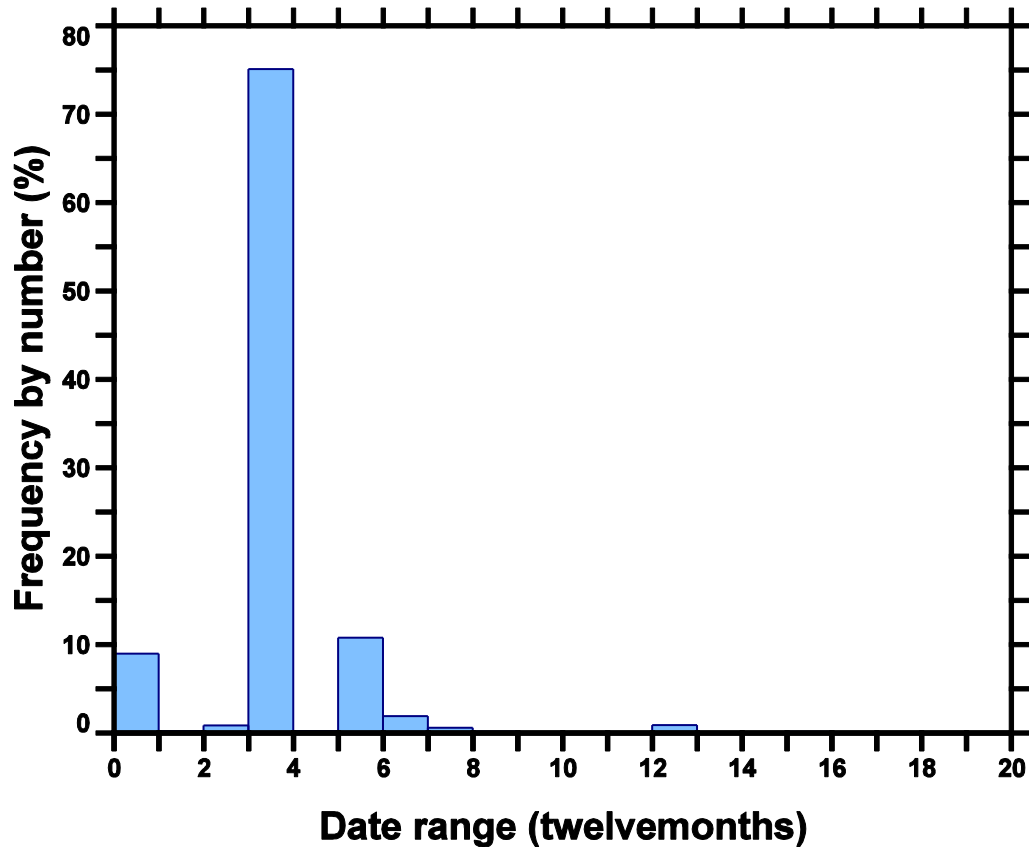
Figure 3. Frequency distribution of date ranges in the RGI. The ranges are numbers of months between BgnDate and EndDate , divided by 12.
