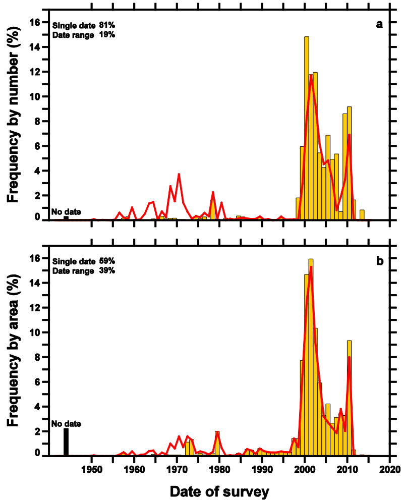
Figure 2. Distribution of dates in the RGI. Line: RGI 4.0; Bars: RGI 6.0. Glaciers with date ranges are assigned with uniform probability to each year of the range. The 633 undated glaciers are confined to regions 10 (Wrangell Island, North Asia), 11 (Italy, Central and Southern Europe) and 19 (Antarctic and Subantarctic).
