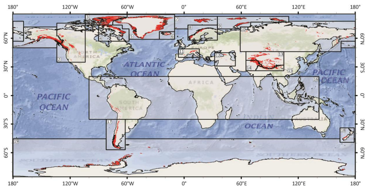
Figure 1. First-order regions of the Randolph Glacier Inventory (version 4.0).
