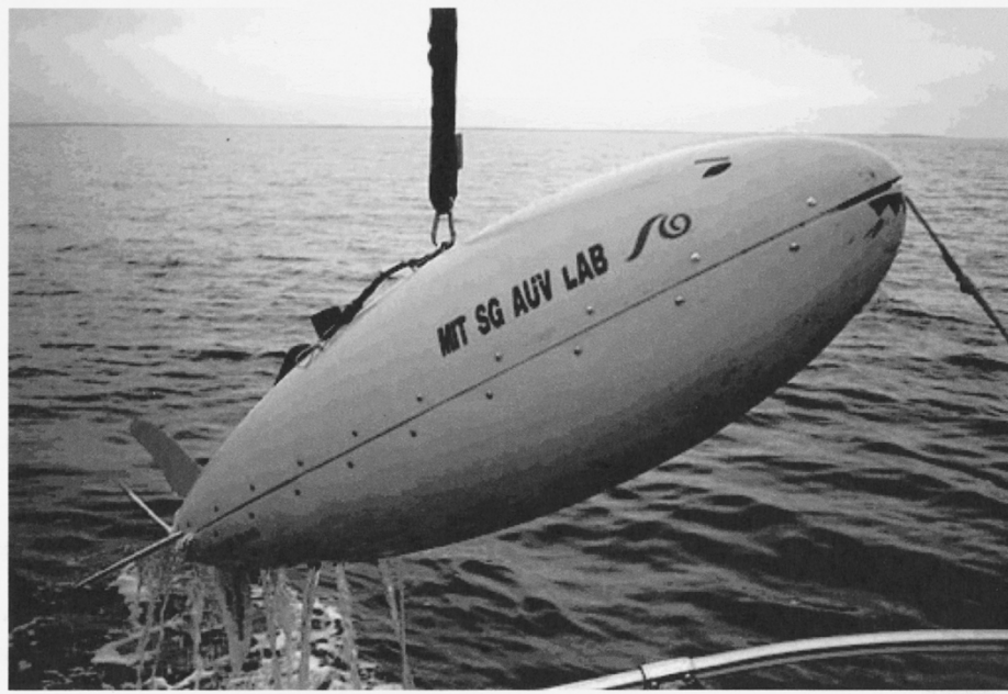
Fig. 1. An Odyssey IIB AUV being recovered after operations.
