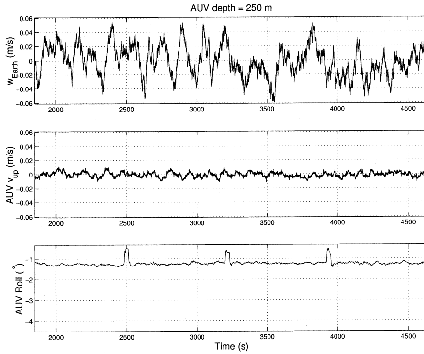
Fig. 18. The Earth-referenced vertical flow velocity w_{\text{Earth}} (the first panel) at the 250-m depth of AUV Mission B9 804 107. In the second panel is the AUV's own vertical velocity. The AUV's roll (the third panel) shows when the vehicle made 90^\circ turns.
