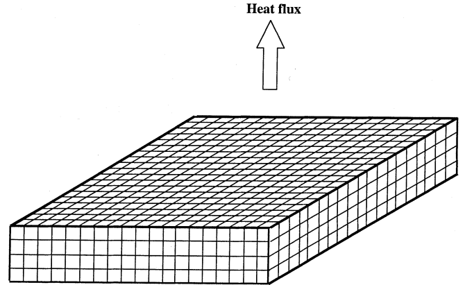
Fig. 8. Illustration of the convection model box. Only the top surface is subjected to a heat flux. The dimension is 200 \times 200 \times 35 with a grid size of 10 m.
