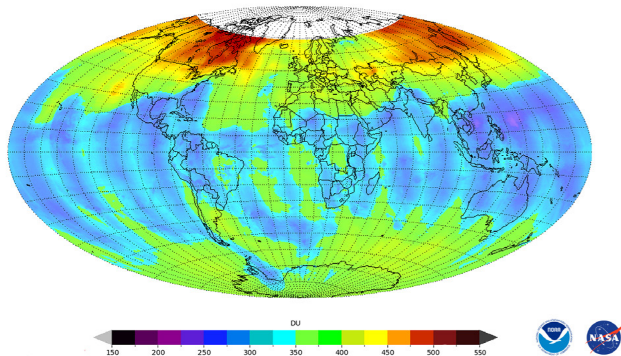
NOAA 21 Total Ozone February 17, 2023
