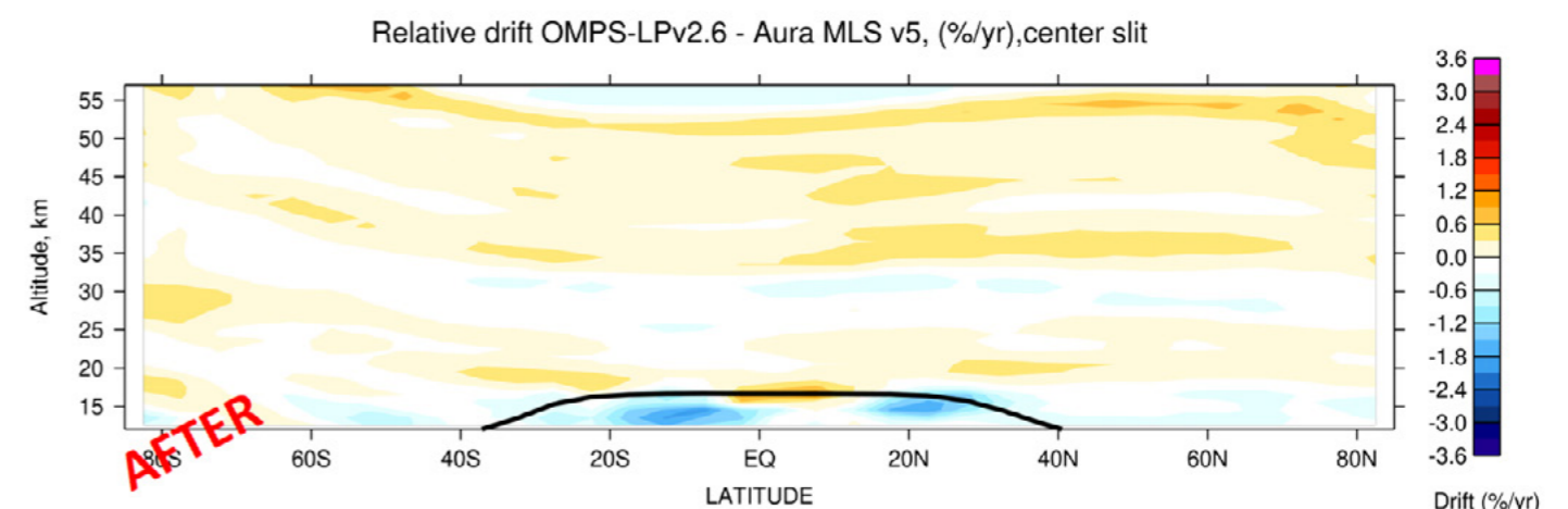
Relative drift in ozone (percent per year) at different altitudes between OMPS LP version 2.6 and Aura MLS version 5. These results are after improvements to the LP retrieval algorithm.
