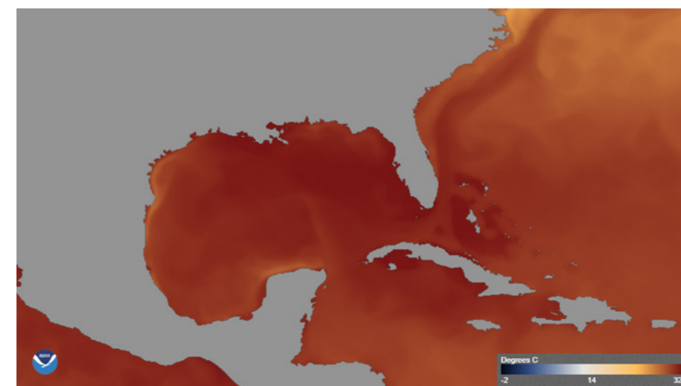
An example of sea surface temperature data that is collected by JPSS satellites. In this example from August 7-13, 2023, higher temperatures are shown by darker red colors around Florida, the Gulf of Mexico, and the Caribbean.
