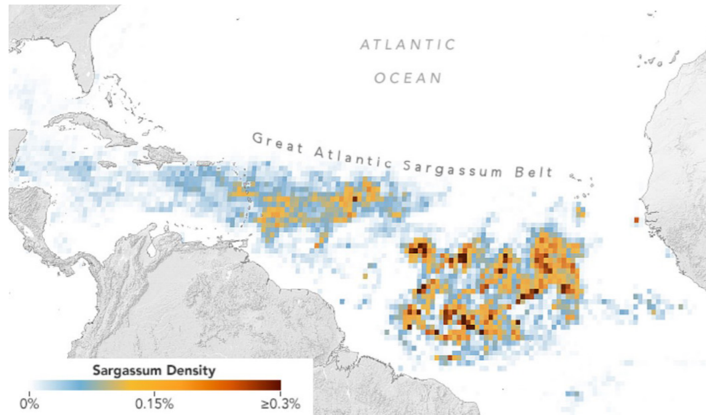
The map above shows Sargassum density in the central Atlantic Ocean (including the Caribbean Sea and Gulf of Mexico) for March 2023. Red and orange areas show where Sargassum densities were the highest, in terms of the percent of the pixel covered with the seaweed. The mass spanned 8,000 kilometers and weighed 13.1 million tons (equivalent to 113,000 blue whales!), a record for this time of year. The data for the map were developed by scientists at the University of South Florida Optical Oceanography Laboratory using data from the Moderate Resolution Imaging Spectrometer (MODIS) onboard NASA Terra and Aqua satellites. Source: NASA Earth Observatory.
