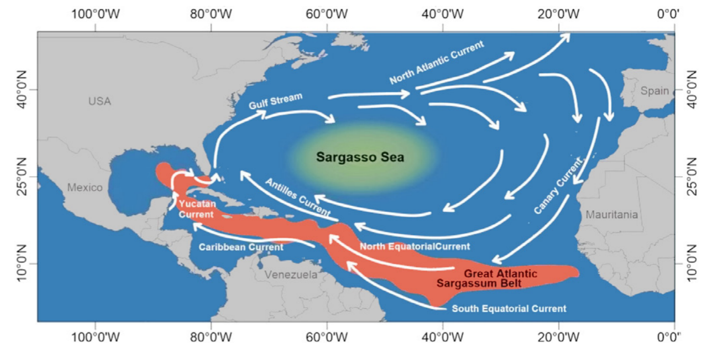
The seasonal Great Atlantic Sargassum Belt stretches from West Africa to the Gulf of Mexico. Credit: López, M.J.L. et al (2021), CC BY 4.0 via Wikimedia Commons.
