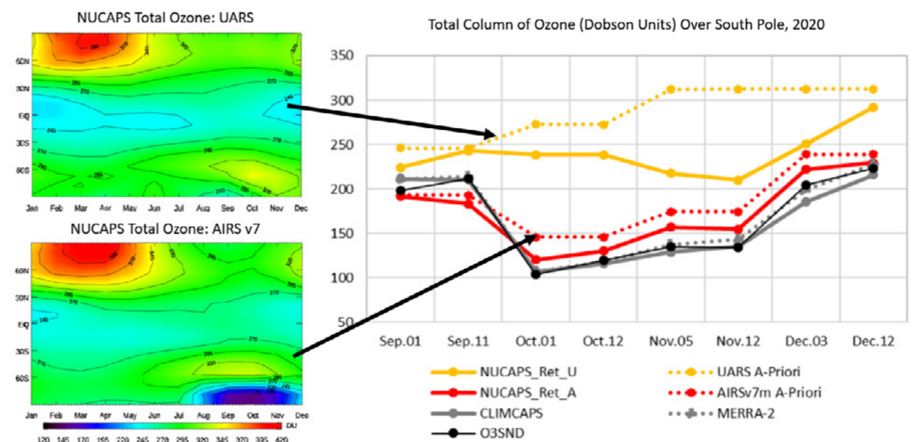
Right: Evaluation of NUCAPS ozone retrievals over Antarctica during the spring to summer transition (September to December 2020. Data is from NUCAPS, CLIMCAPS, ozonesondes, and MERRA-2. Top left: NUCAPS ozone retrievals from UARS (ozone a priori validated maturity version, top). Bottom left: NUCAPS ozone retrievals from AIRS (ozone new a priori, bottom).
