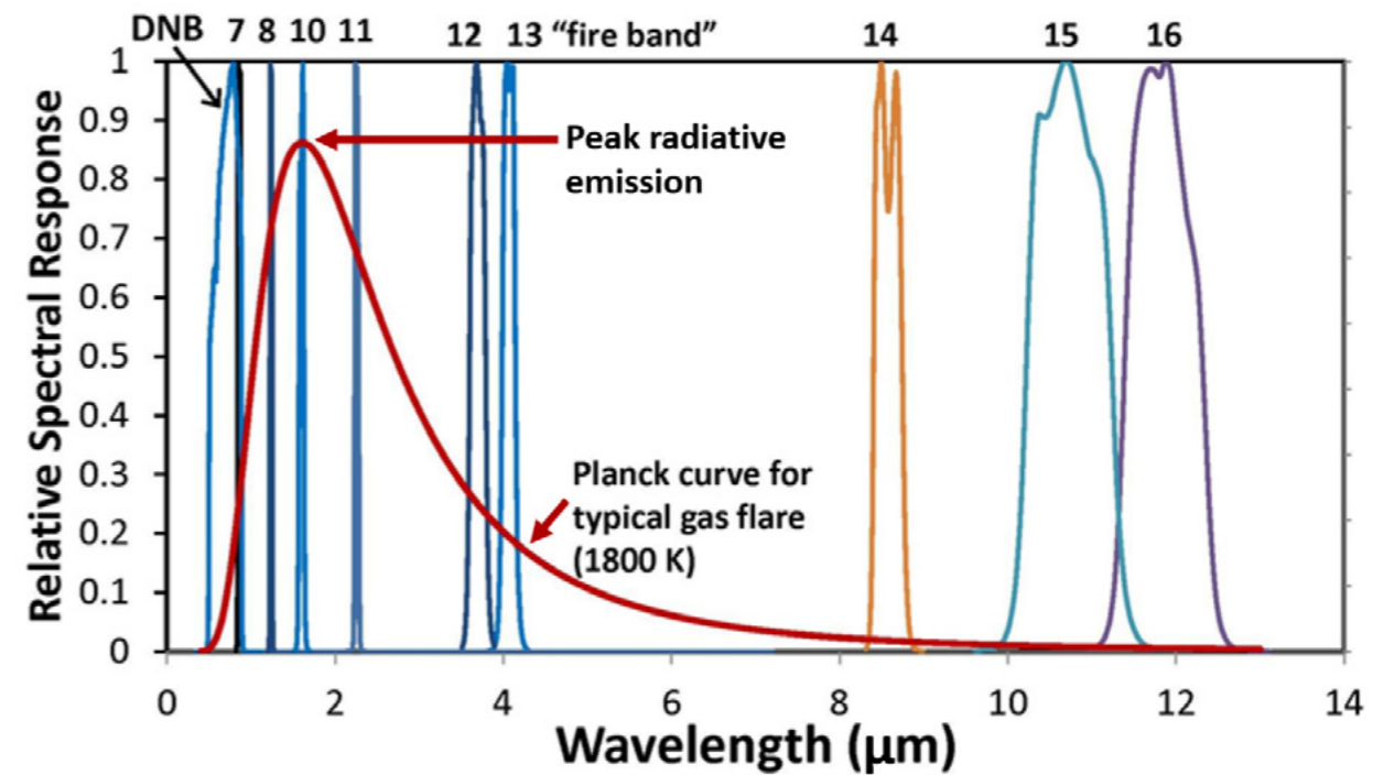
Relative spectral response of VIIRS M-bands and the Planck curve of typical gas flares at 1800 Kelvin. DNB refers to the VIIRS Day/Night Band. Source: Elvidge et al, 2016.
