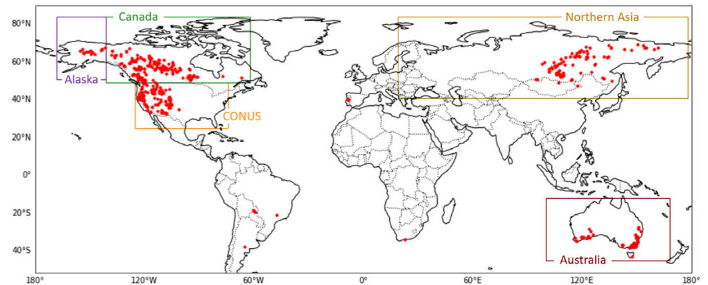
The distribution of pyroCb events recorded from 2013-2021.
