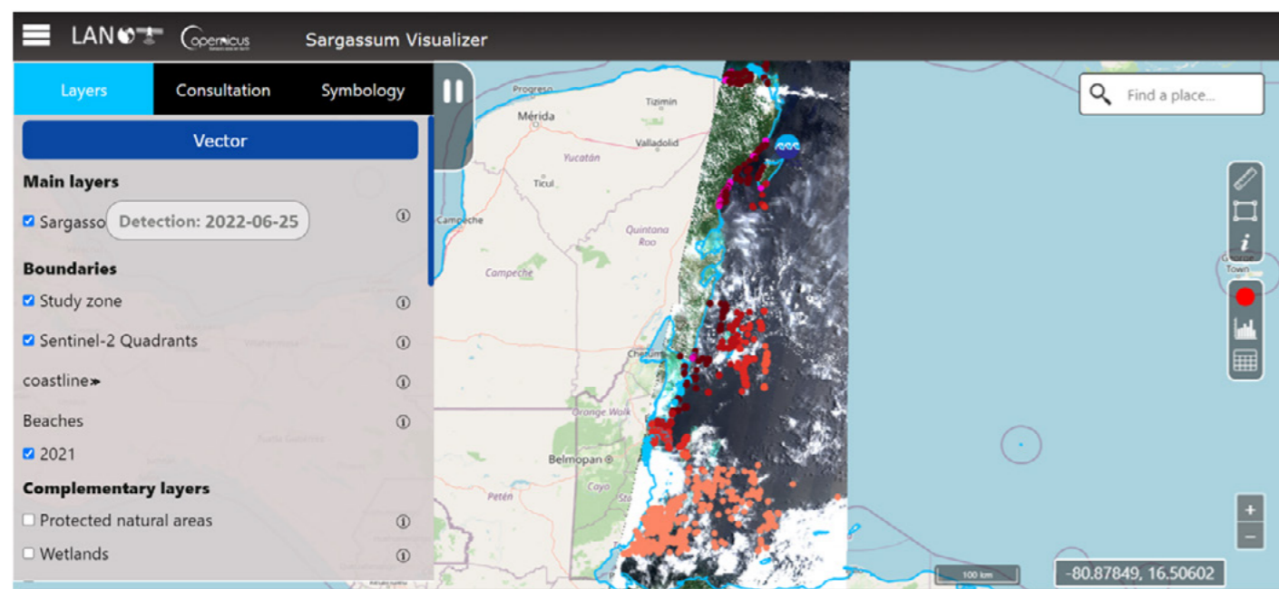
Screenshot of LANOT's Sargassum Visualizer. Sargassum detections are depicted by red and orange dots.
