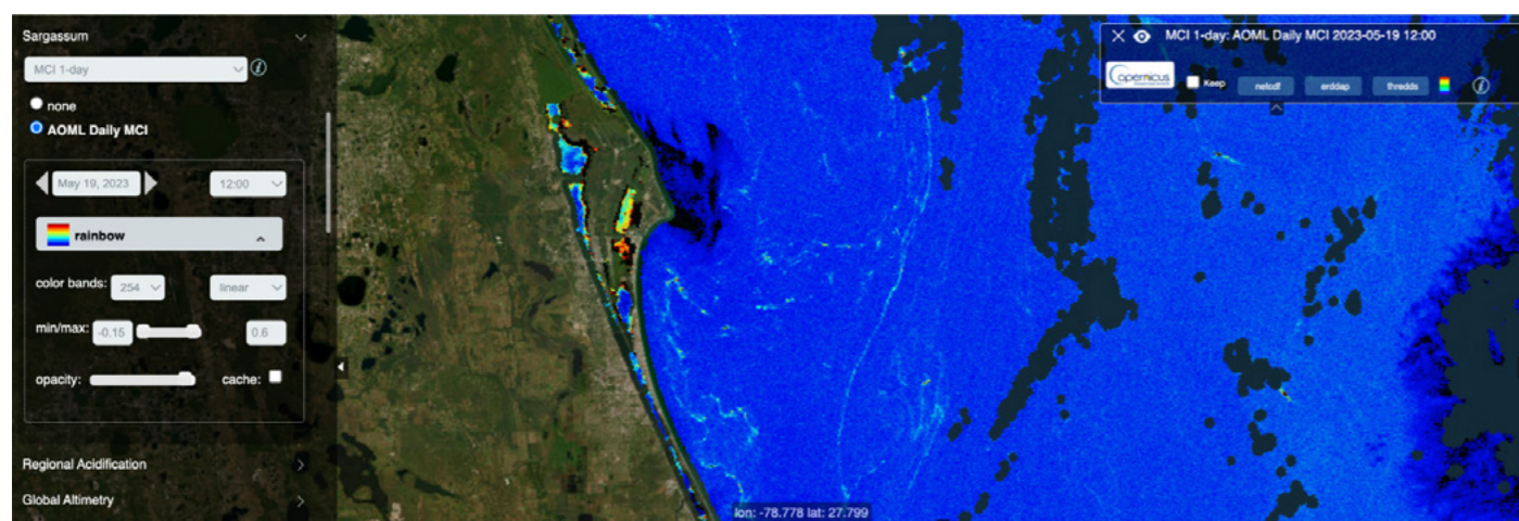
Screenshot of Ocean Viewer showing the presence of Sargassum along Central Florida on May 19, 2023. The Maximum Chlorophyll Index (MCI) identifies those areas with high concentrations of chlorophyll. We can see the characteristic lines of high MCI along the coast, indicating the presence of Sargassum . There are also high values of MCI in the lagoons near Cape Canaveral that do not represent Sargassum , but rather, coastal eutrophic areas. Source: Ocean Viewer
