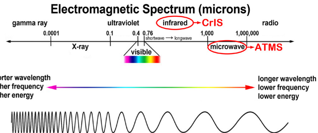
Comparison of wavelength, frequency, and energy for the electromagnetic spectrum. The JPSS CrIS and ATMS instruments measure infrared and microwave wavelengths, respectively. Credit: NASA Imagine the Universe.
