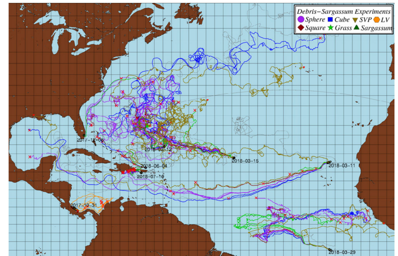
Trajectories of drifters deployed in the debris- Sargassum experiments conducted by the AOML Physical Oceanography Division.
