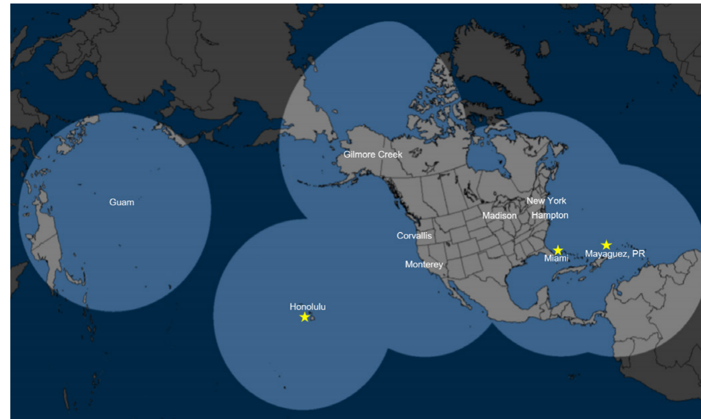
Direct Broadcast receiving stations in the U.S. Yellow stars indicate sites where NRL is retrieving data: Miami, Puerto Rico, and Honolulu.
