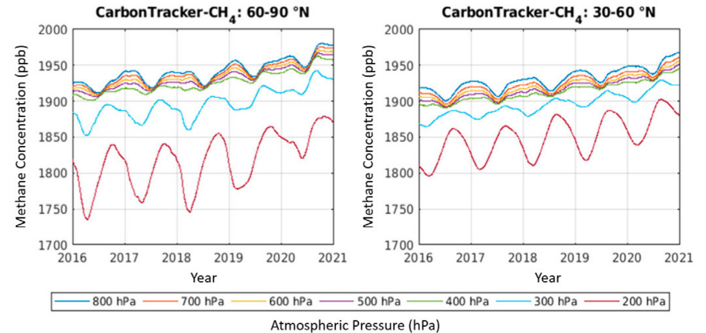
Time Series of Zonally Averaged Methane From CarbonTracker-CH 4 at 200-800 hPa for Zonal Bands 60-90°N and 30-60°N
