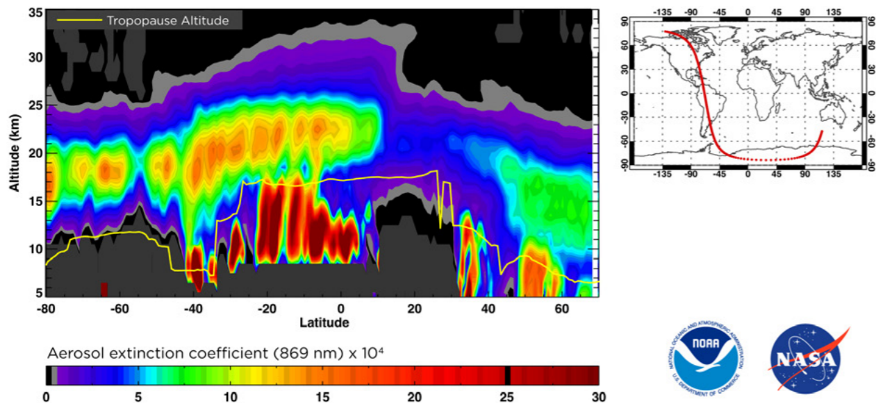
Figure 3: The OMPS limb instrument on the NOAA-21 satellite on Feb. 17 detected sulfates remaining from the January 2022 Hunga-Tonga volcanic plume eruption between an altitude of 12 to 15 miles in the tropics. Credit: NASA/NOAA/JPSS
