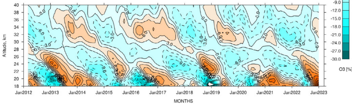
De-seasonalized ozone anomalies (in %) over the equatorial latitudes (5°S to 5°N) from OMPS LP version 2.6 (top) and Aura MLS version 5 (bottom). The instruments had very similar responses in ozone to an anomalous QBO event in late 2015 and 2016.
