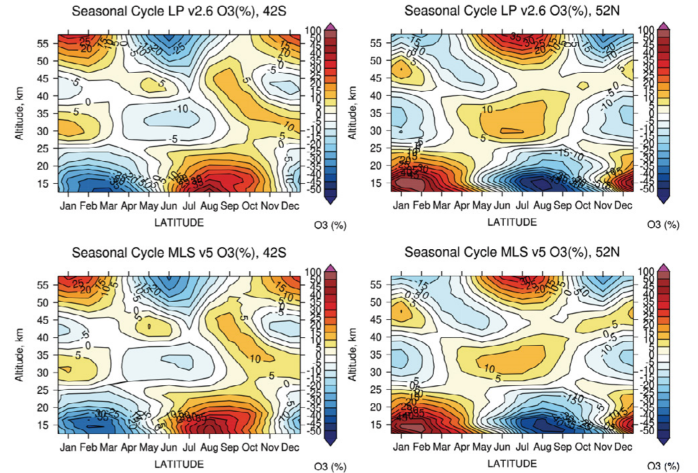
Seasonal ozone cycles (shown in % from the annual mean) derived from OMPS LP version 2.6 (top row) and Aura MLS version 5 (bottom row) as functions of month and altitude for 42°S (left) and 52°N (right).
