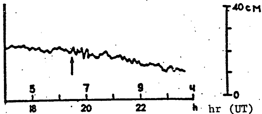
Figure 21: Record of tsunami of September 27, 1971 in Nevel'sk [Shchetnikov, 1981].
