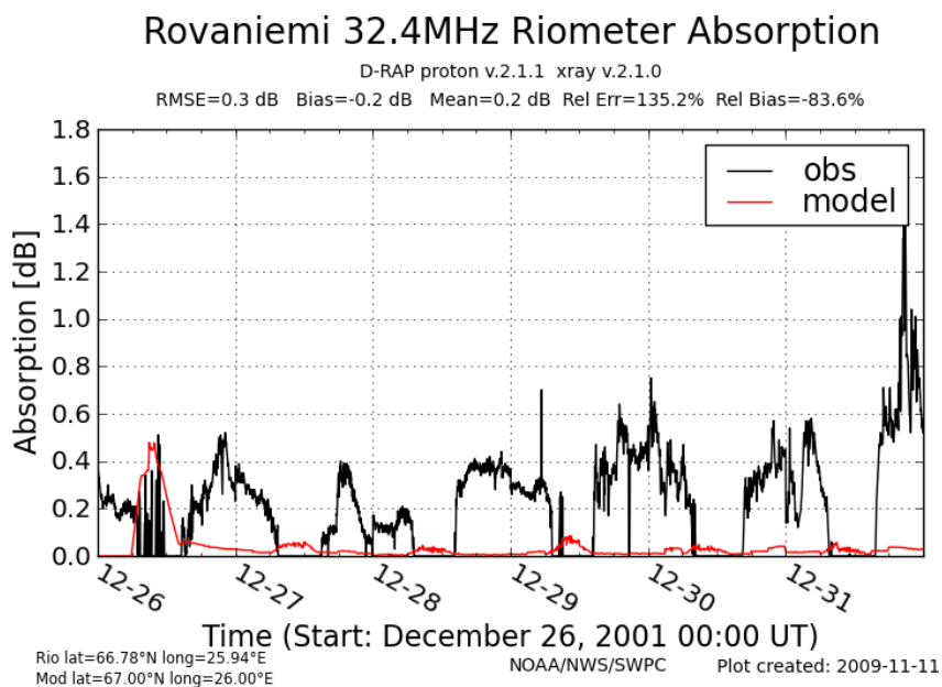
Figure 5. Comparison of model and riometer absorption at Rovaniemi for period 10.
