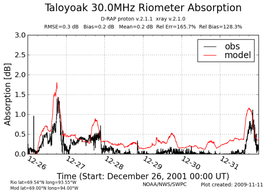
Figure 6. Same as in Fig. 5 but at Taloyoak.
