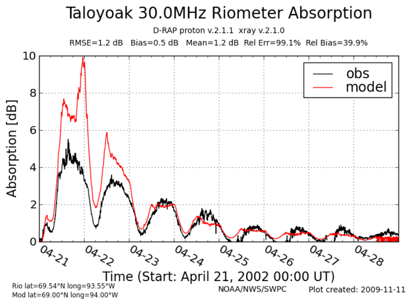
Figure 3. Comparison of model and riometer absorption at Taloyoak for period 11.
