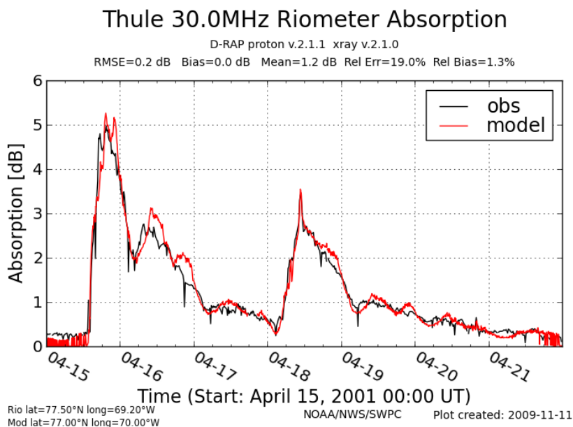
Figure 1. Comparison of model and riometer absorption at Thule for period 5.
