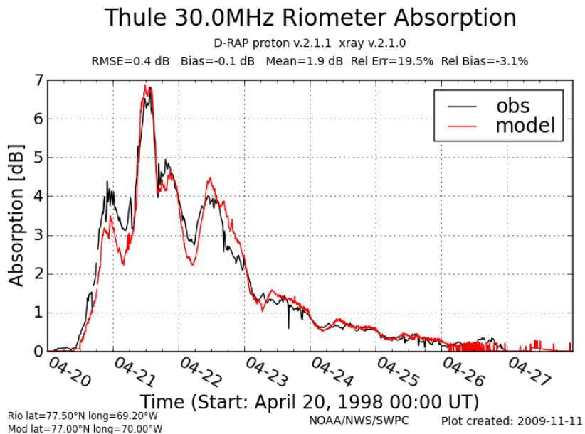
Figure 7. Comparison of model and riometer absorption at Thule for period 1.
