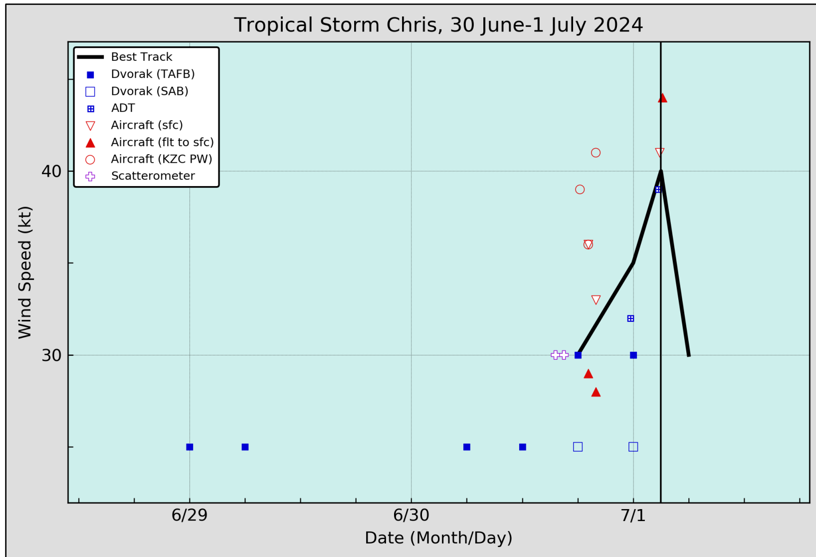
Figure 2. Selected wind observations and best track maximum sustained surface wind speed curve for Tropical Storm Chris, 30 June–1 July 2024. Aircraft observations have been adjusted for elevation using 90% and 75% adjustment factors for observations from 700 mb and 925 mb, respectively. Advanced Dvorak Technique estimates represent the Current Intensity at the nominal observation time. Dashed vertical lines correspond to 0000 UTC, and solid vertical lines correspond to landfalls.
