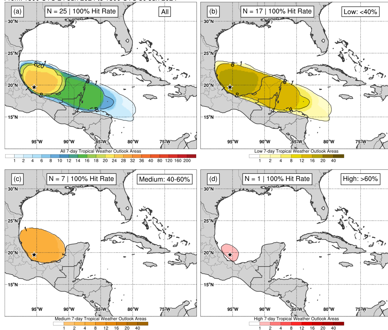
Figure 5. Composites of 7-day tropical cyclone genesis areas depicted in NHC’s Tropical Weather Outlooks prior to the formation of Tropical Storm Chris for (a) all probabilistic genesis categories, (b) the low (<40%) category, (c) medium (40–60%) category, and (d) high (>60%) category. The location of genesis is indicated by the black star. Note that the single genesis forecast in the high category (panel d) was issued at the time Chris is analyzed to have become a tropical cyclone.
