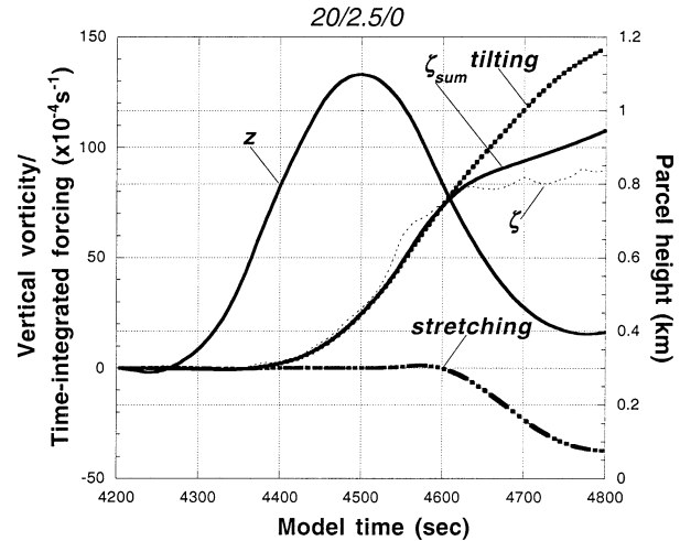
FIG. 7. Time series of parcel height ( z ; km), vertical vorticity ( \zeta ; \text{s}^{-1} ), and the time-integrated contributions to vertical vorticity from the tilting and relative vorticity-stretching terms [ \text{s}^{-1} ; see Eq. (4.1)], along the backward trajectory denoted as “B” in Fig. 6. The sum of the tilting and stretching terms is plotted as \zeta_{\text{sum}} .
